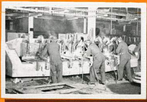
Welding Fixture
