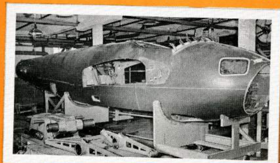
The Boxing Fixture
