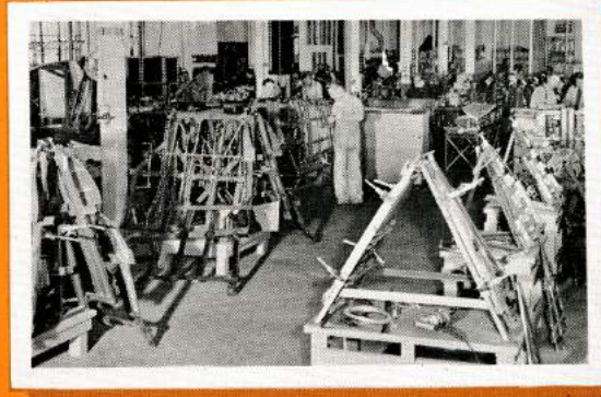
Jigs to Shape Nacelles
