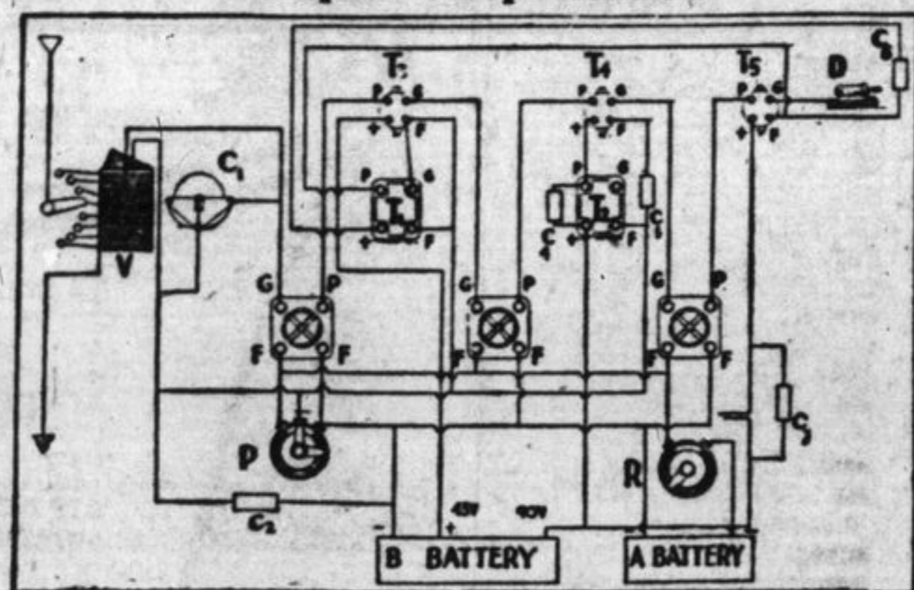
Hookup Diagram of a Three-Tube Reflex Set.
