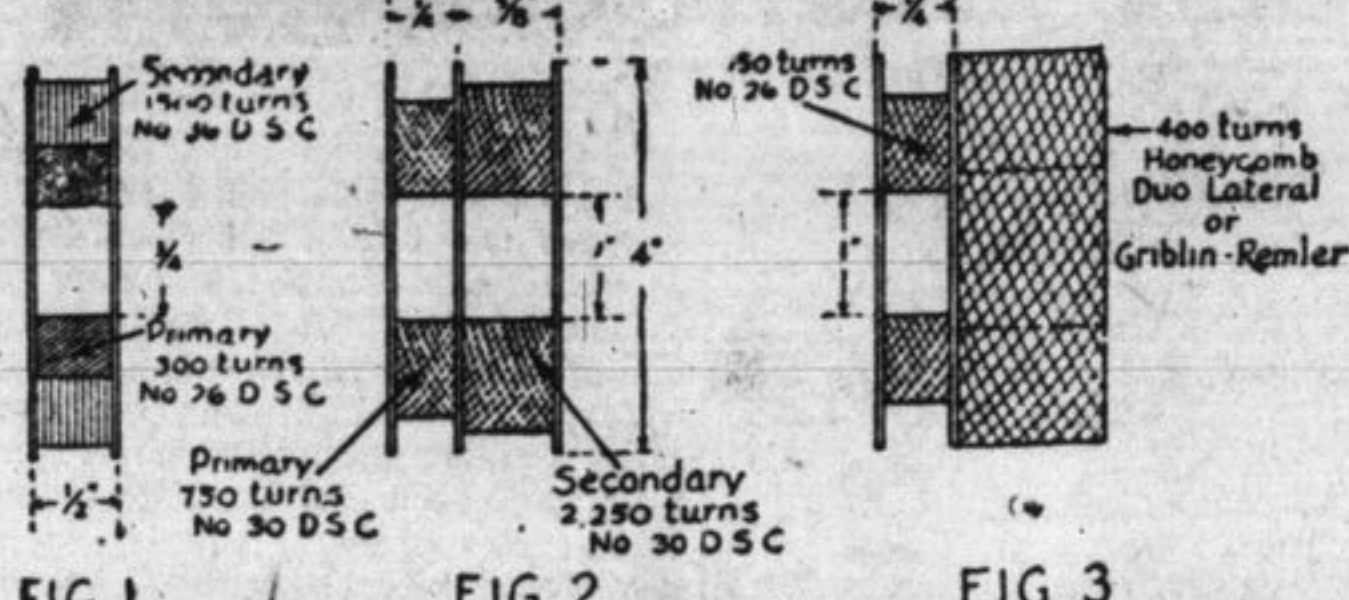
FIG 1 FIG 2 FIG 3 Design Data on Intermediate Transformers
