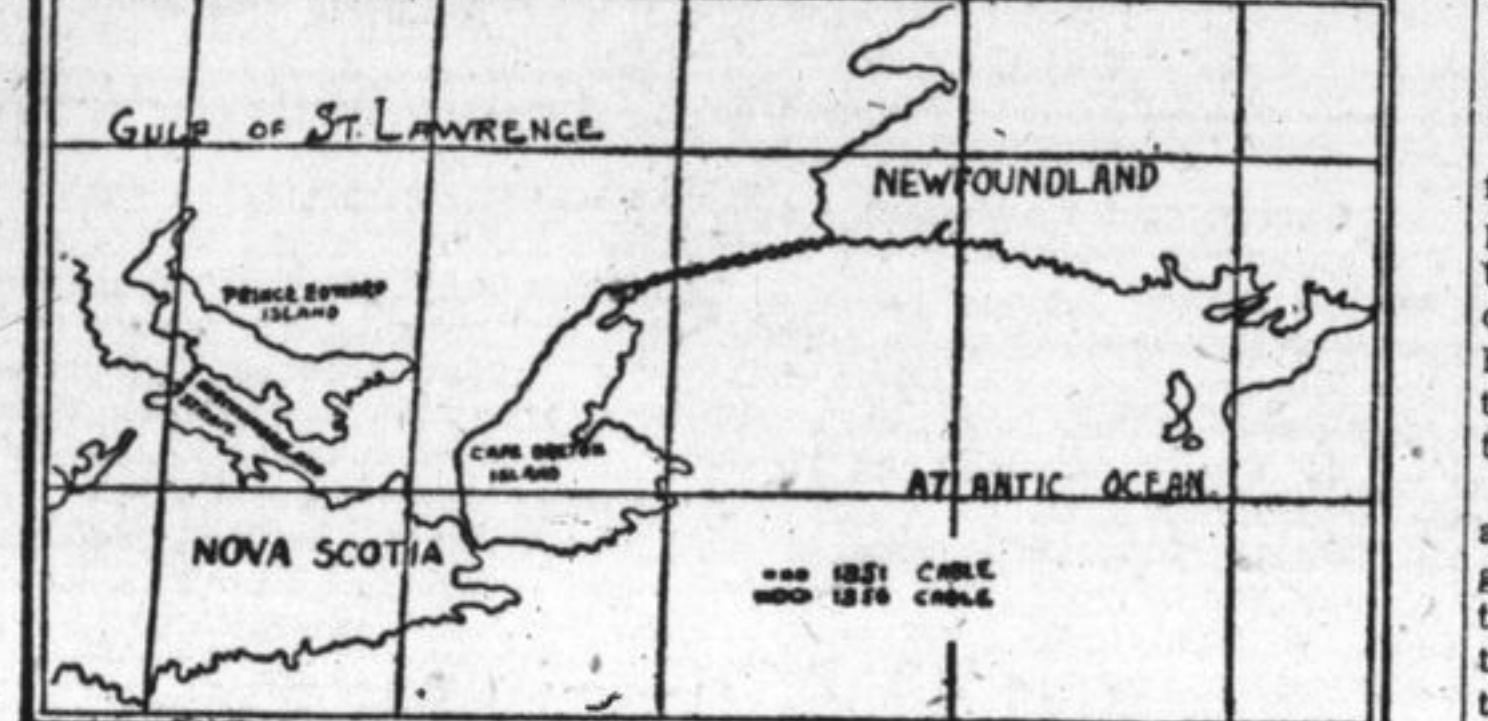
MAP OF THE FIRST SUBMARINE CABLE Also the first cable of any length that preceded the idea of the Atlantic Cable, which was originated and engineered in Canada.
