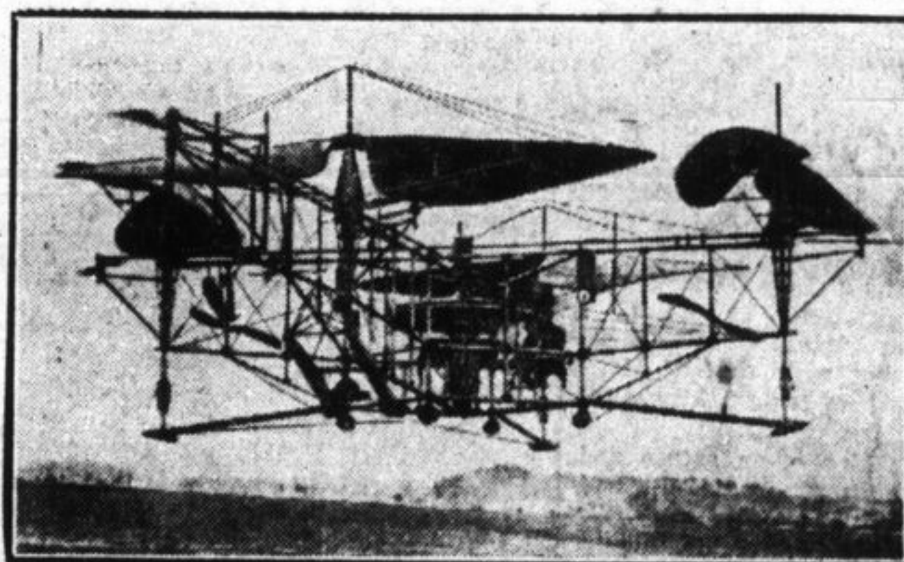
The new Oehmichen helicopter trials at Les Breuils, France, are reported to be the most successful of any before attempted. The pilot did not try for altitude, but confined his flying from ten to fifteen feet from the ground
