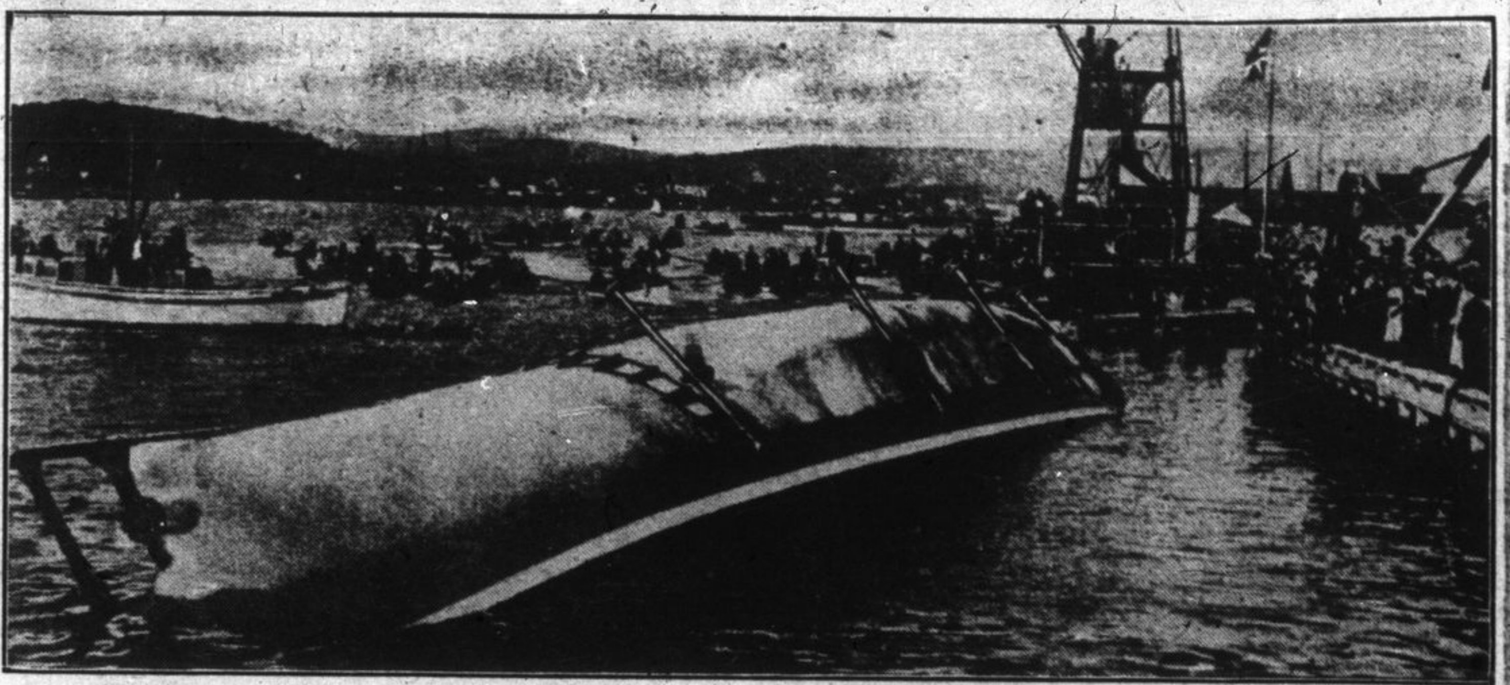
Boat built of concrete under the direction of the United States Shipping Board is launched at Savannah, G. The craft is sent bottom side up into the water, where it almost immediately rights itself, owing to the low centre of gravity, and the water is then pumped out.
