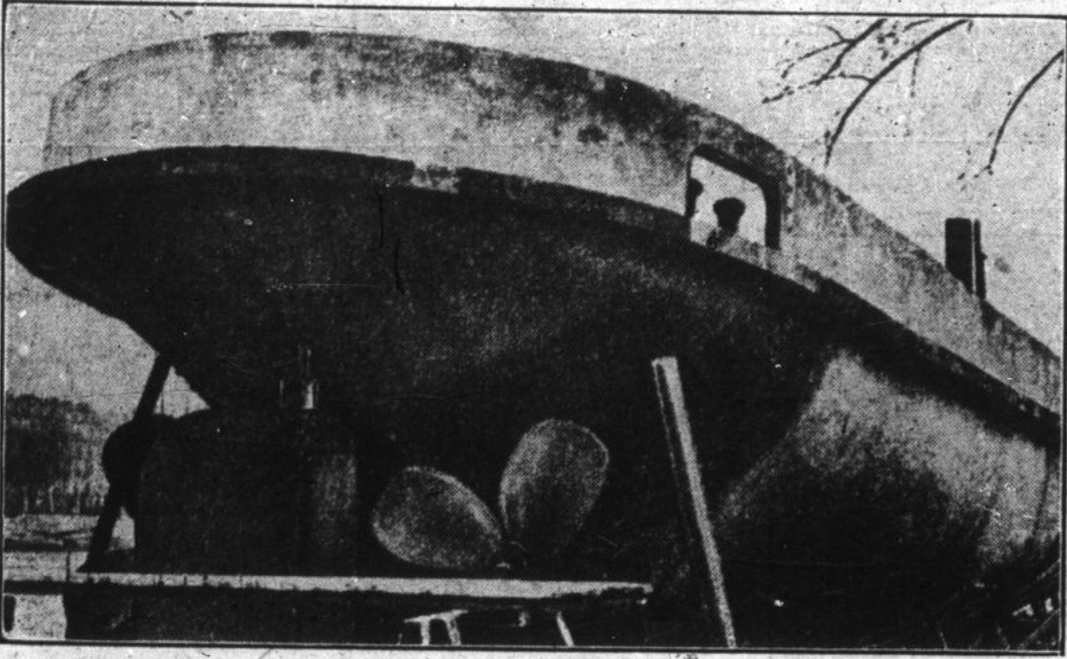
After part of one of the twin-screw ships under construction at Ivory-on-the-Seine, near Paris. The need for coastwise and river vessels has caused the French to use concrete in shipbuilding as yielding the quickest results.
