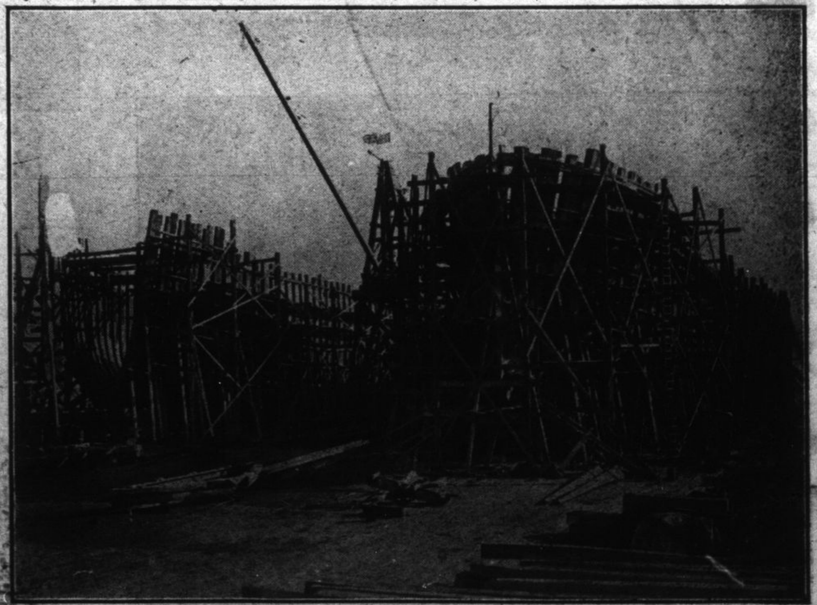
Wooden ships at the Western Canada Shipyards, at Vancouver, in the course of construction.
