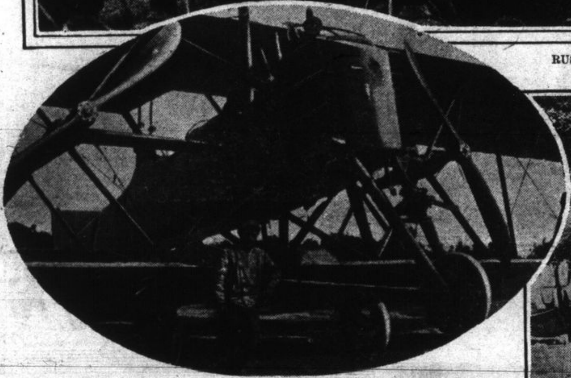
Wireless on aircraft. Showing (in front) the small screw which, actuated by the air, drives the dynamo for the electric current.
