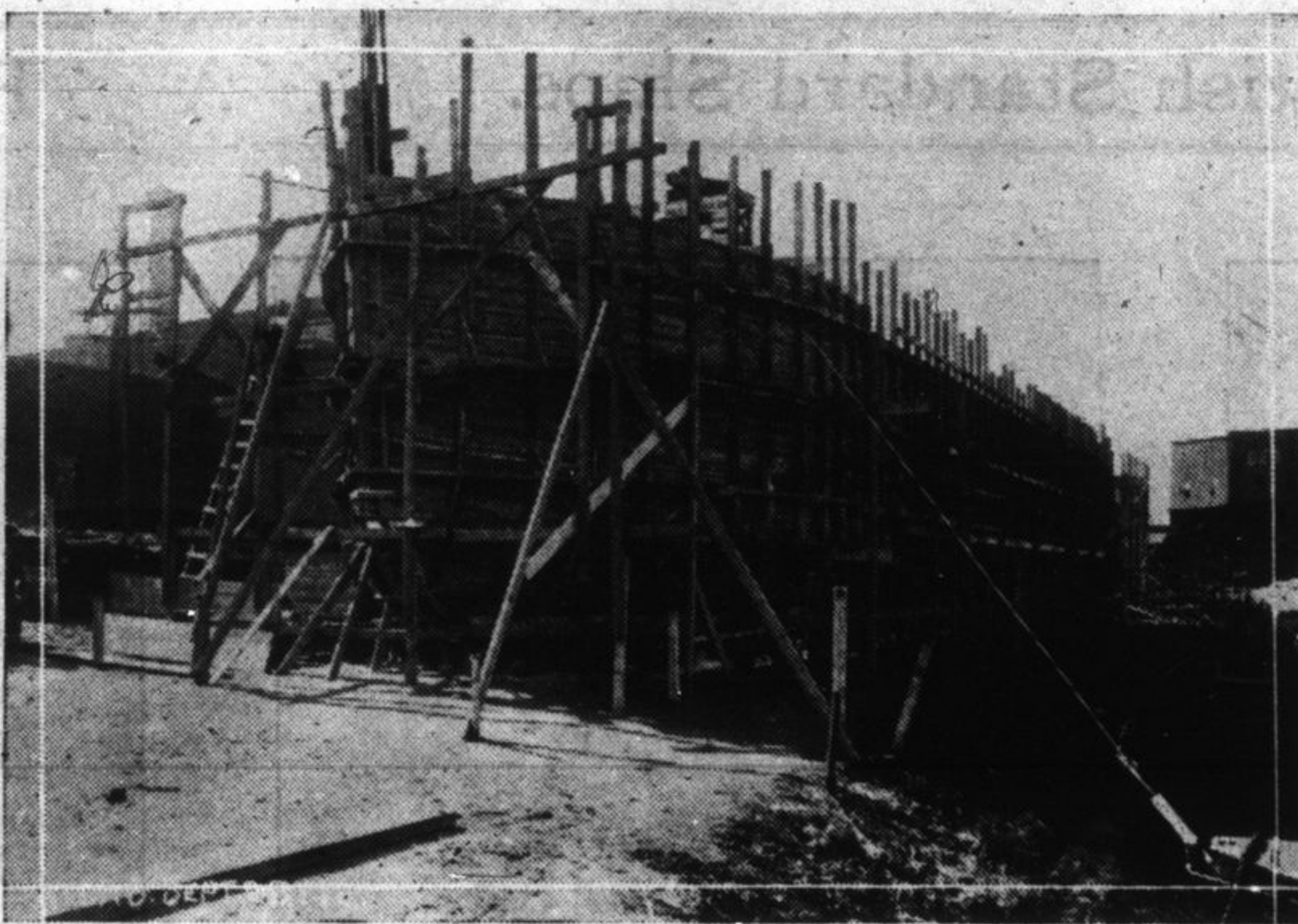
Concrete ships are being built for Canada. The first self-propelling concrete boat is now under construction in Montreal. When completed it will be thoroughly tested for lake, coastwise or ocean service. A concrete hull can be completed in ten weeks.
