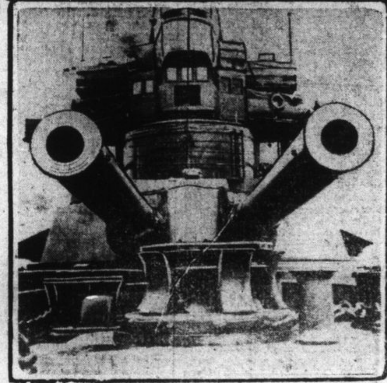
The Monarch, a North Sea unit, was built in 1912 and is of the Orion class. She carries ten 13.5 in. guns, four 3 prs., sixteen 4 in. three torpedo tubes. The small views show two of her formidable looking guns.
