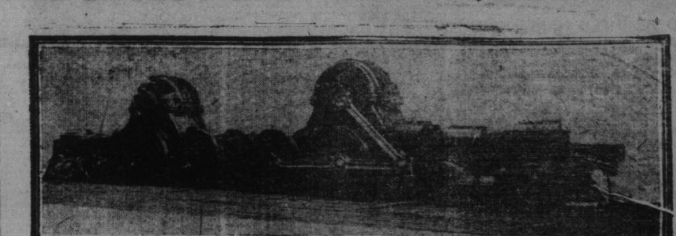
CHASSIS OF ELECTRIC LOCOMOTIVE NO. 2292, TO BE USED IN THE NEW YORK TUNNELS.
