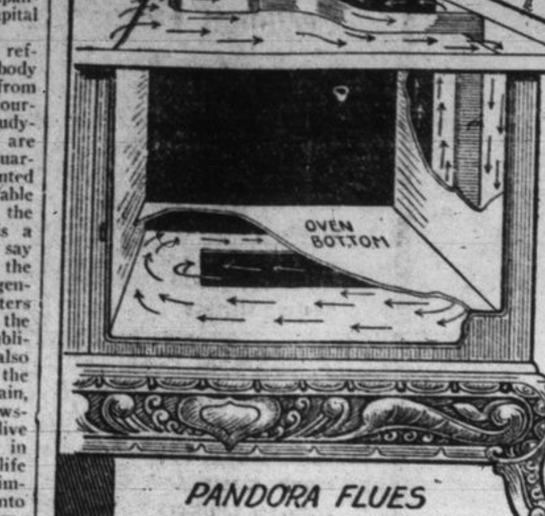
PANDORA FLUES. Arrows show direction of heat.
