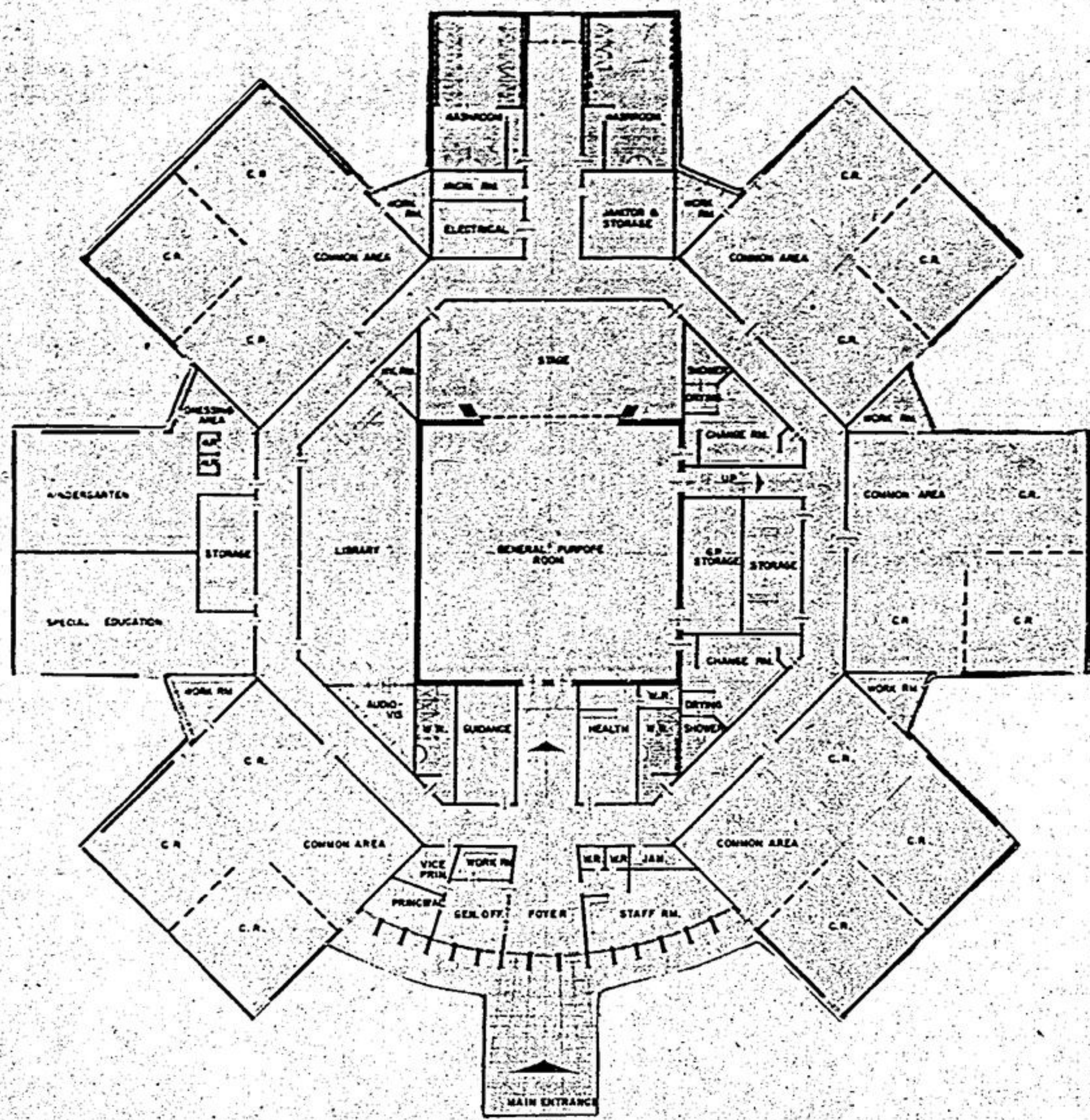
Sketch drawing of new public school plan for Whitchurch Twp.
