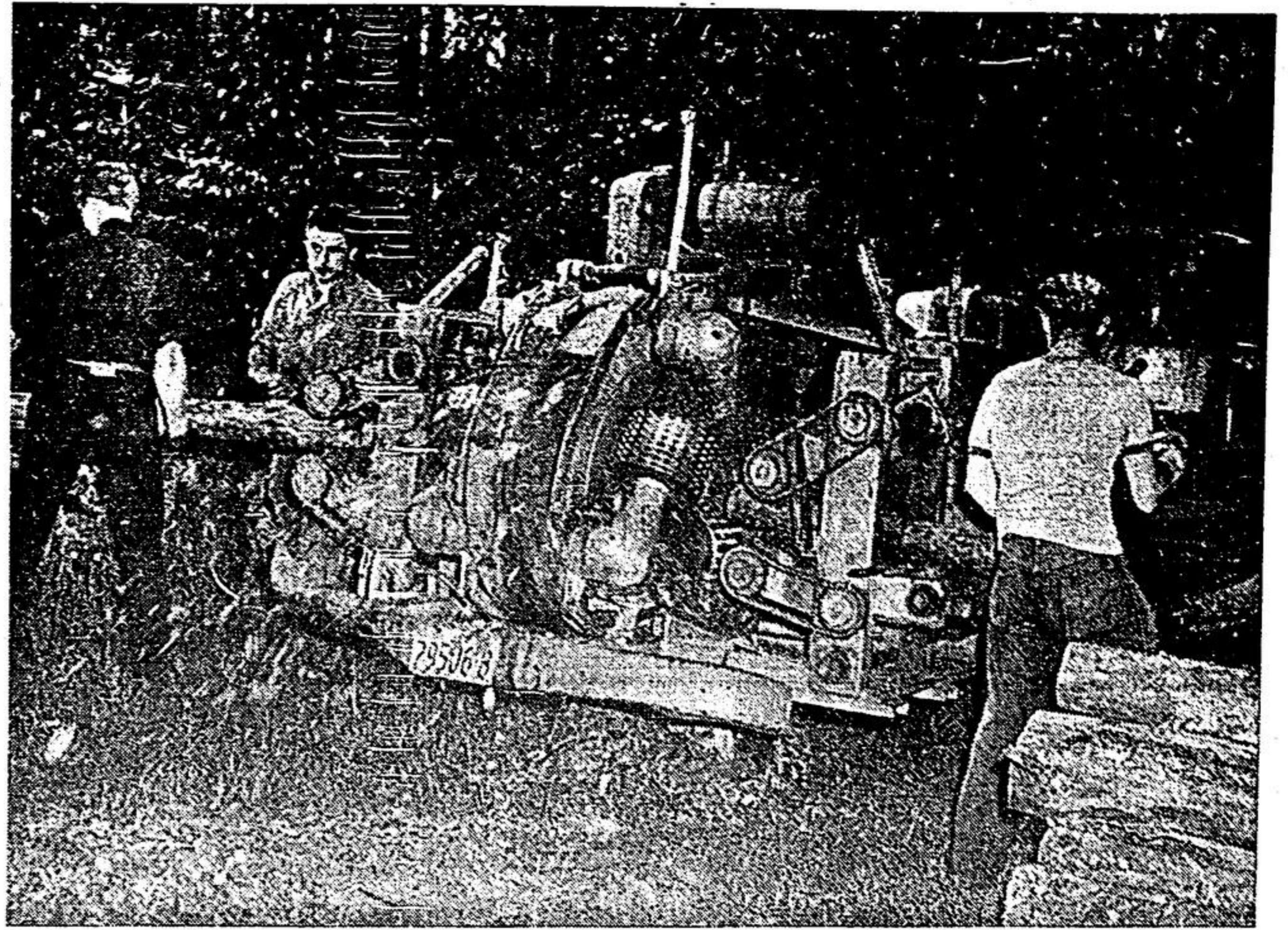
Visitors watch demonstration of a Cambio Barker, owned by the Wagner Pulpwood Industries, and used for debarking wood. This machine debarks an average of 80 cords per day.
