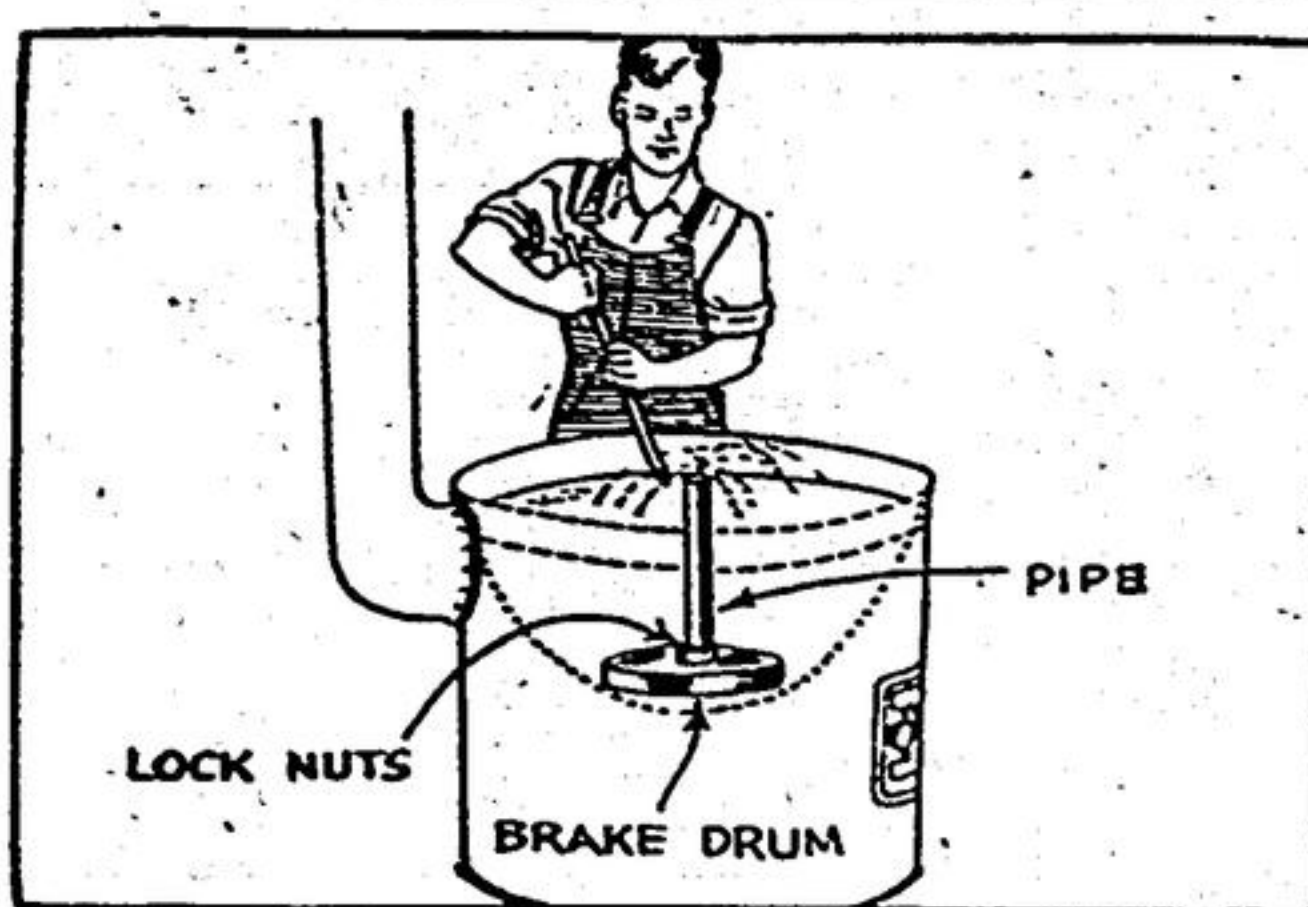
COOKER... Inexpensive percolator cooks feed for poultry or livestock. Pipe is threaded and locked in opening of drum by a nut on each side. Liquid contacts top of food as well as bottom, thus reducing cooking time.
