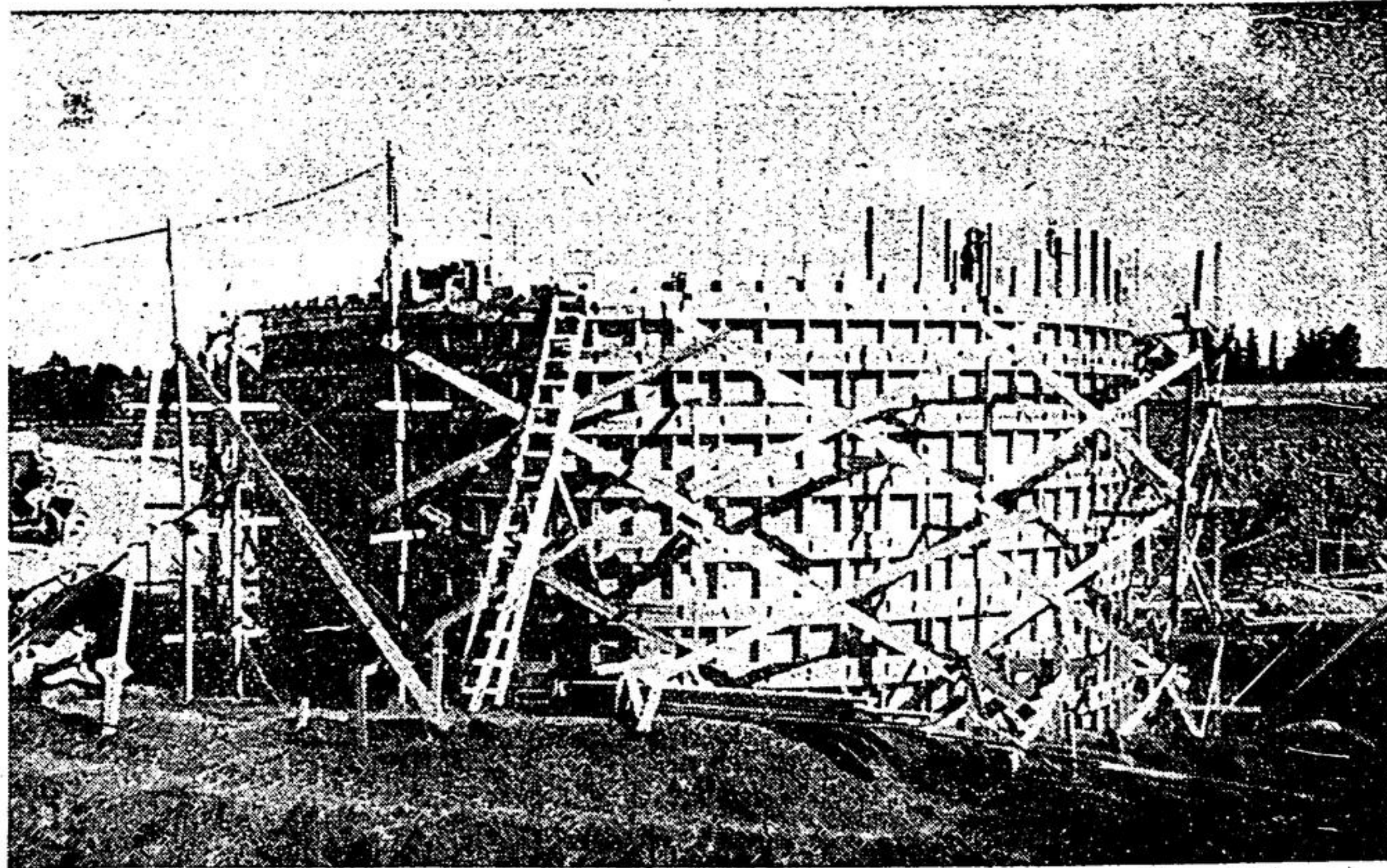
The huge sludge "digester" pictured above is all part of Stouffville's integral sewerage system which is now under construction.
