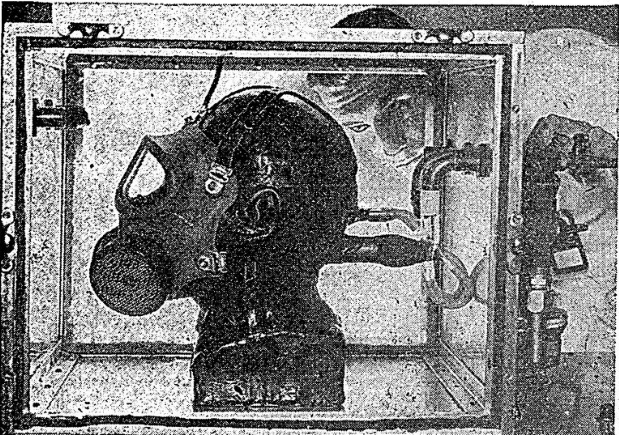
A 'HOT HEAD' —This rubber head devised for use at a plutonium plant in Richland, Wash., tests the face masks that must protect workers from "hot" radio-active contamination. Human breathing is simulated by multiple pumps fitted to the device. A filter inside the "windpipe" collects radioactive particles that find their way in.
