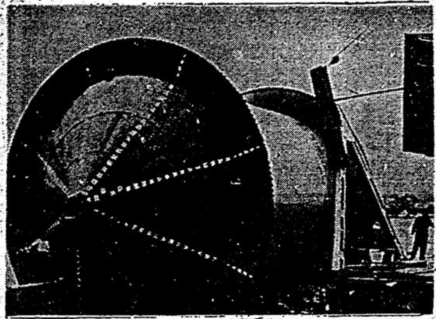
This huge drum was used by Allied engineers to unwind a 67-mile length of pipe across the English channel to carry oil to the armies fighting on the continent.
