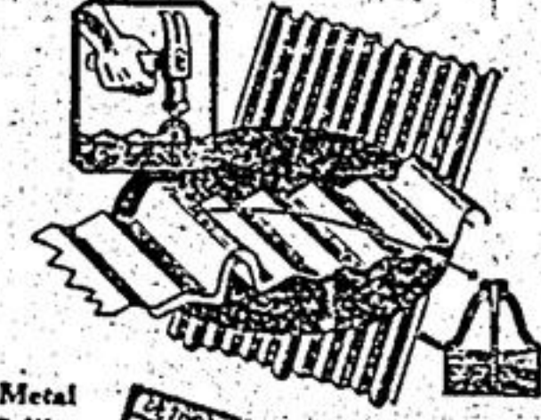
Below—A "close-up" of RIB-ROLL, showing LED-HED nail and wide side lap. When nailed this joint is invisible from even a short distance away.
