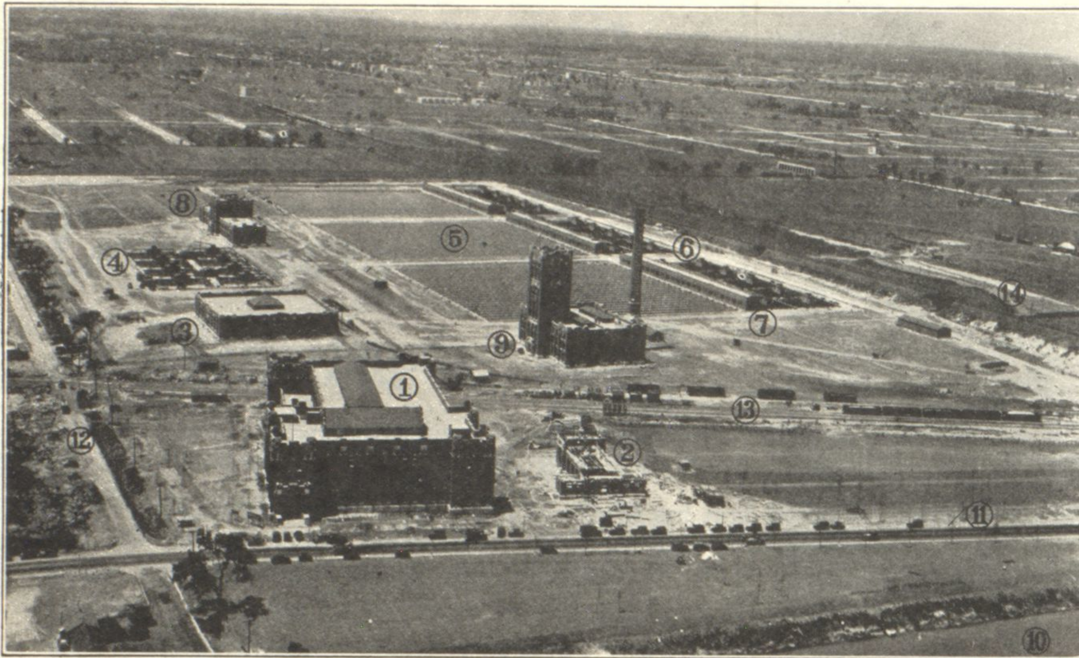
The sanitary district's mammoth north side sewage treatment plant at Oakton street and McCormick boulevard has been opened. This plant serves all the territory in Cook county between Fullerton avenue and the north boundary of the county. This picture shows a bird's-eye view of the plant. 1. is the main pumping station and blower house, 2. is the outdoor sub-station, 3. the grit chamber and coarse screen house, 4. the preliminary settling tanks, 5. the aeration tanks, 6. the final settling tanks, 7. the operating galleries, 8. the main building, 9. the service building, 10. the drainage canal, which will no more carry untreated sewage, 11. is McCormick boulevard, 12. is Howard street, 13. is the C. & N. W. railroad and 14. is the "L."
