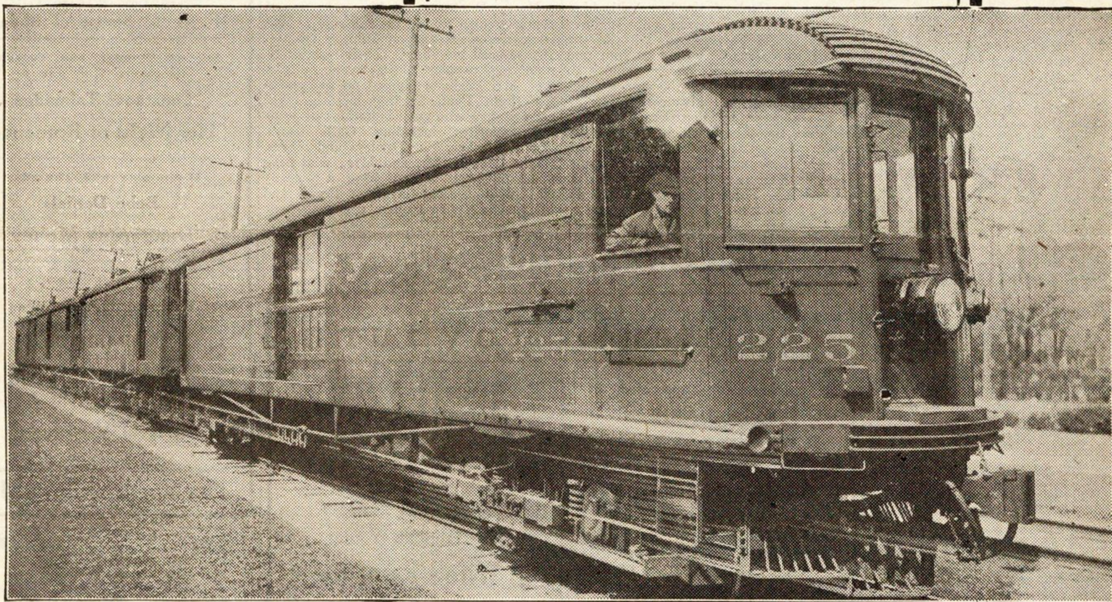
A Merchandise Despatch Train
