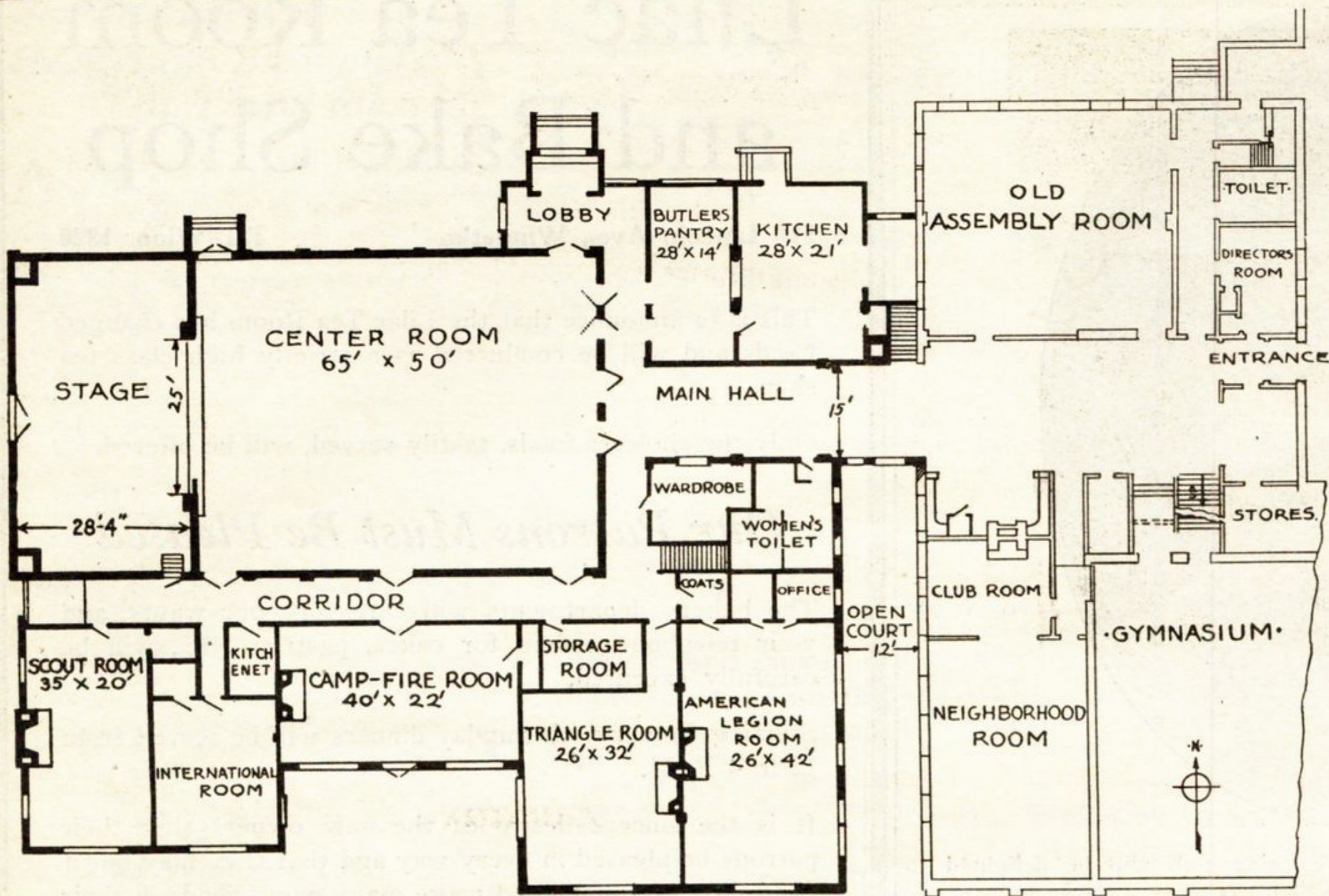
EXISTING COMMUNITY HOUSE.
