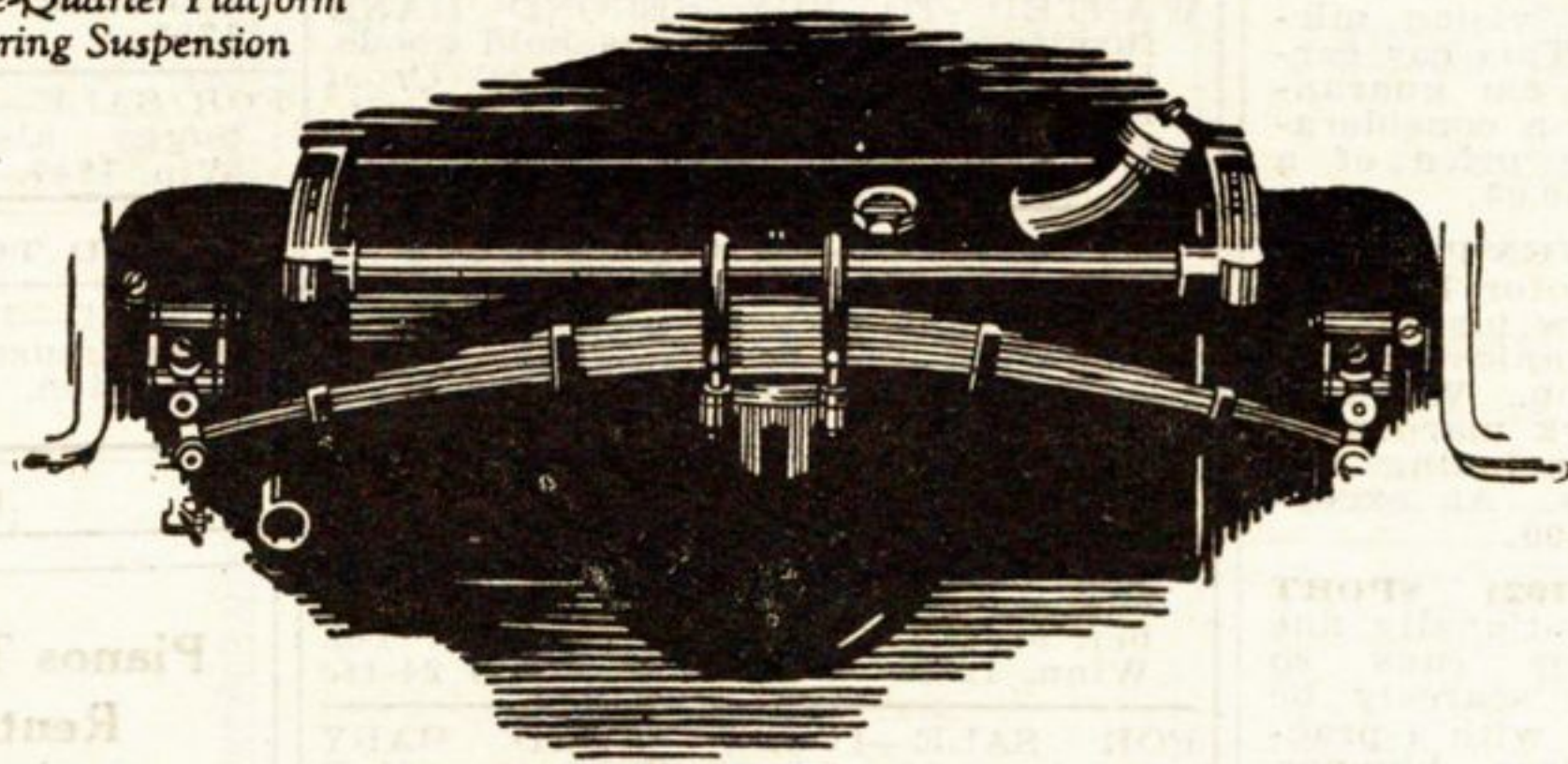
A Rear View of the Cadillac Three-Quarter Platform Spring Suspension
