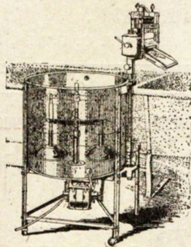
Easy Vacuum Washer with Gas Burner
