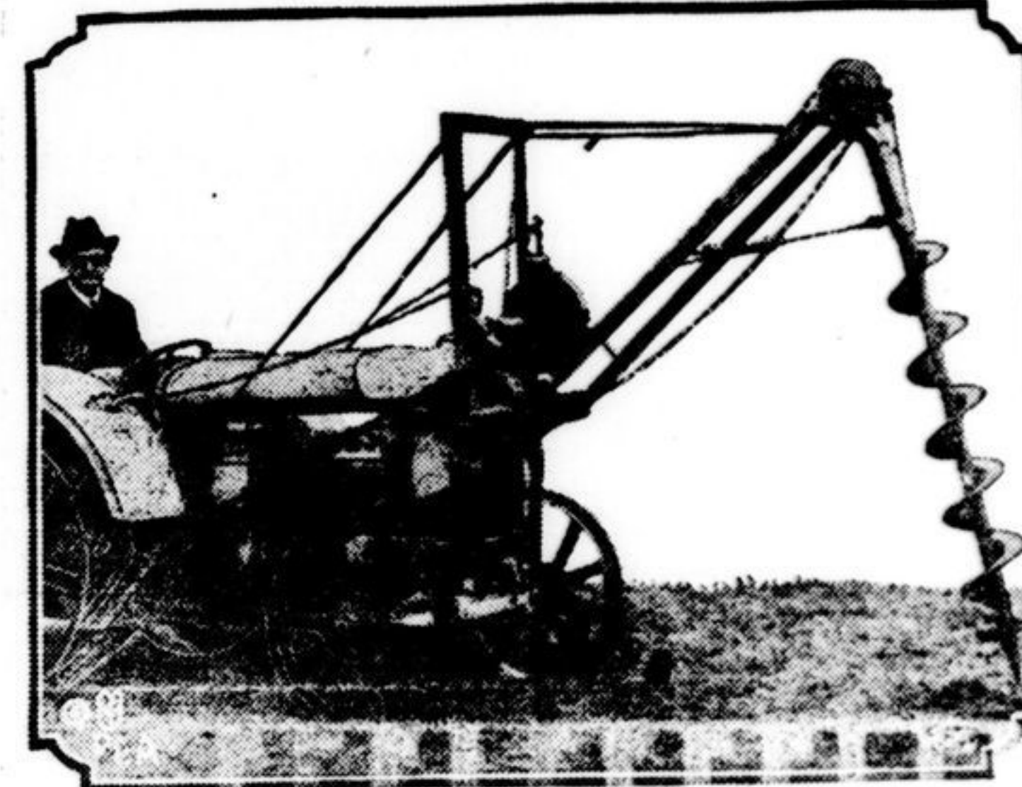
POST-HOLE drilling need no longer be tedious, slow work. An Ohio inventor has devised the above illustrated augur that can be operated by any farm tractor and will dig a three-foot hole, nine inches in diameter, in thirty seconds. A pull on a rod is sufficient to start the augur downward and another pull stops it at the required depth and brings it to the original starting point. The inventor built his original model from twenty-three pieces of farm machinery.
