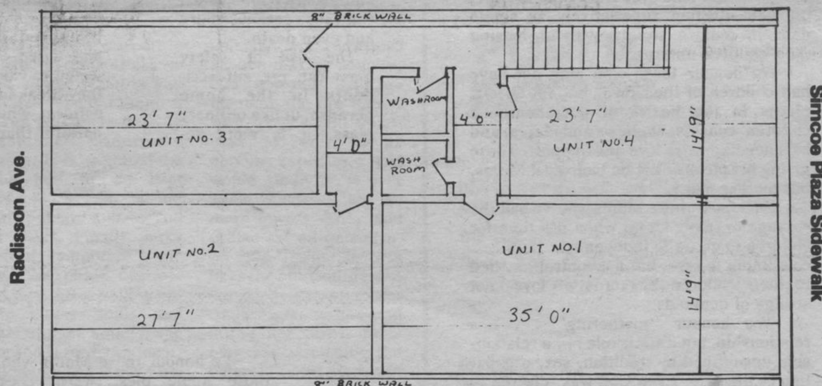
SECOND FLOOR
