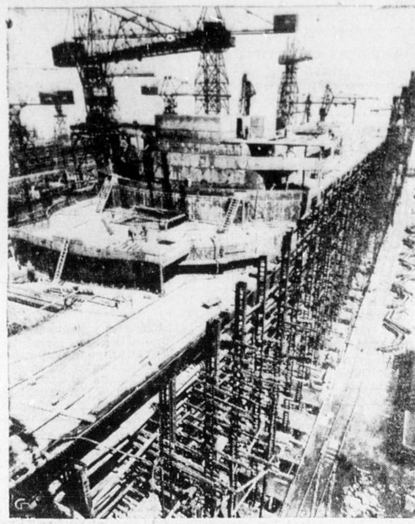
Work is being rushed on the new Cunard-White Star liner, Mauretania, rapidly nearing completion at the shipyards of Birkenhead, England, so that the launching can take place, as scheduled, on July 28.
