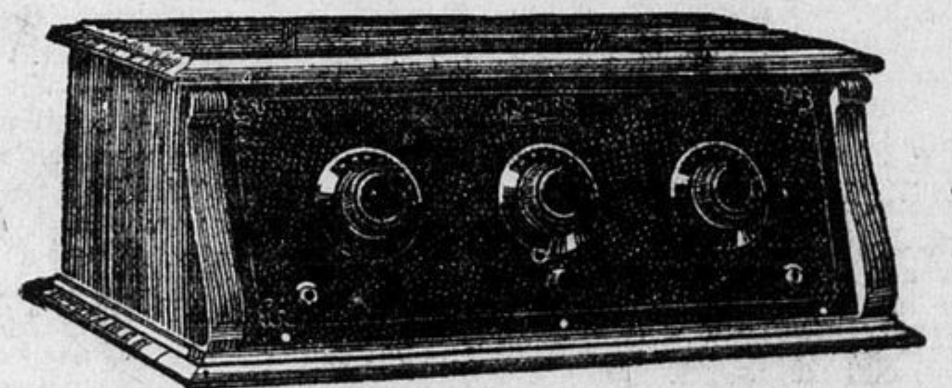
ROGERS SUPER A/C TABLE MODEL-5 TUBE Type 120—Without loud speaker. Equipped with 5 A/C Tubes and Rogers Patented Power Unit, eliminating "A" and "B" Batteries. Complete ready to plug into light socket.
