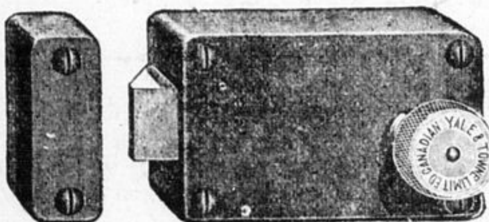
No. 26 Yale Rim Night Latch. Operated from outside by key, from inside by knob. Bolt may be held back by stop. 2x3 1/4 x 3/4 in. japanned iron case and strike. Nickel-plated steel turn knob and key plate, wrought brass tube, bronze-plated iron bolt, back set 2 1/2 in., two nickel-plated solid steel keys, six changes. Reversible for doors 1 1/4 in. thick Price..
