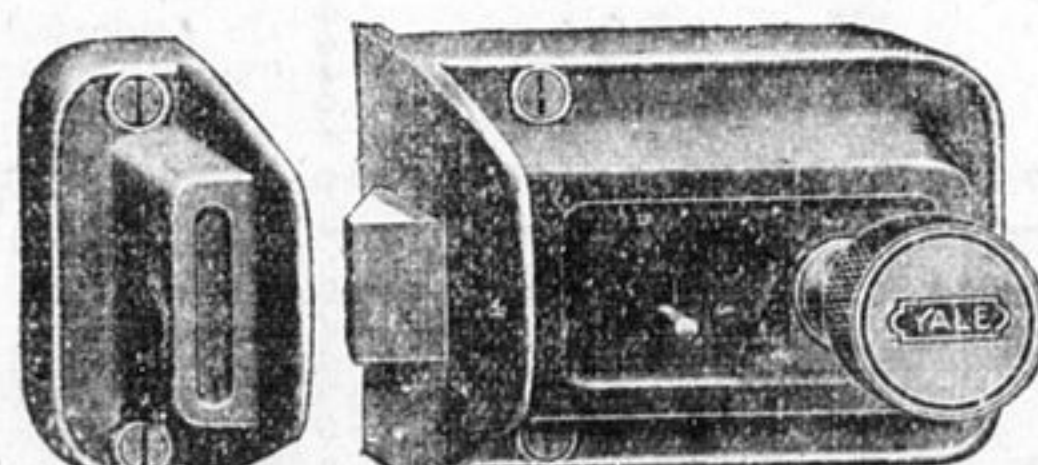
No. 33 Yale Tubular Night Latch. Operated from outside by key, from inside by knob. 2 1/4 x 3 x 3/8 in. japanned iron case, buffed bronze cylinder and knob, bronze stop, bronze-plated steel tube and iron bolt. Back set 2 in. Reversible for doors 7/8 in. to 1 1/2 in. thick. Each in paper box complete with Screws. Price $3.00
