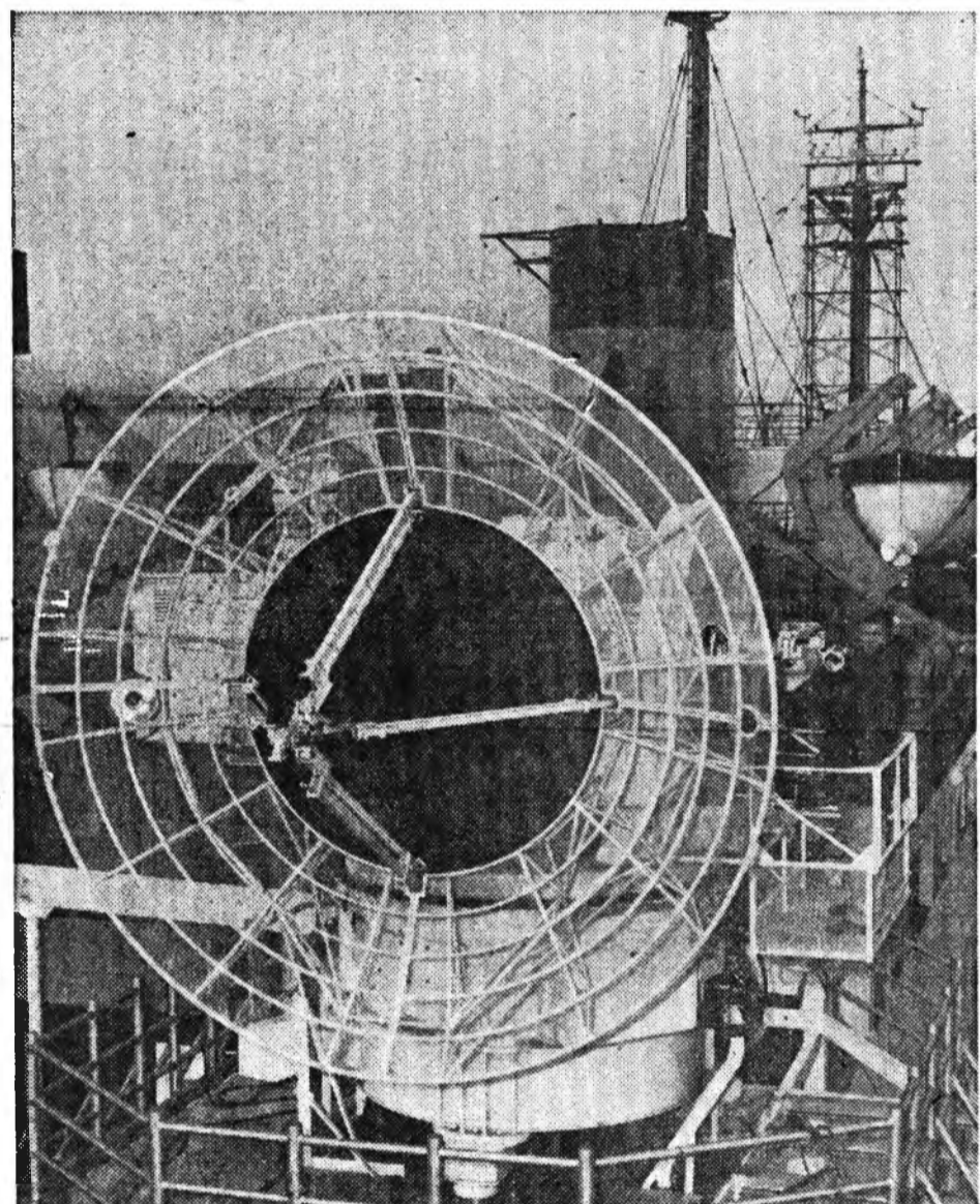
THE LARGEST? 'EYE-EYE' —This is one of two tracking radar antennae on the American Mariner , a new missile-research patrol vessel in the South Atlantic. The largest such afloat, RCA-designed system can "see" any missiles at distances of hundreds of miles.
