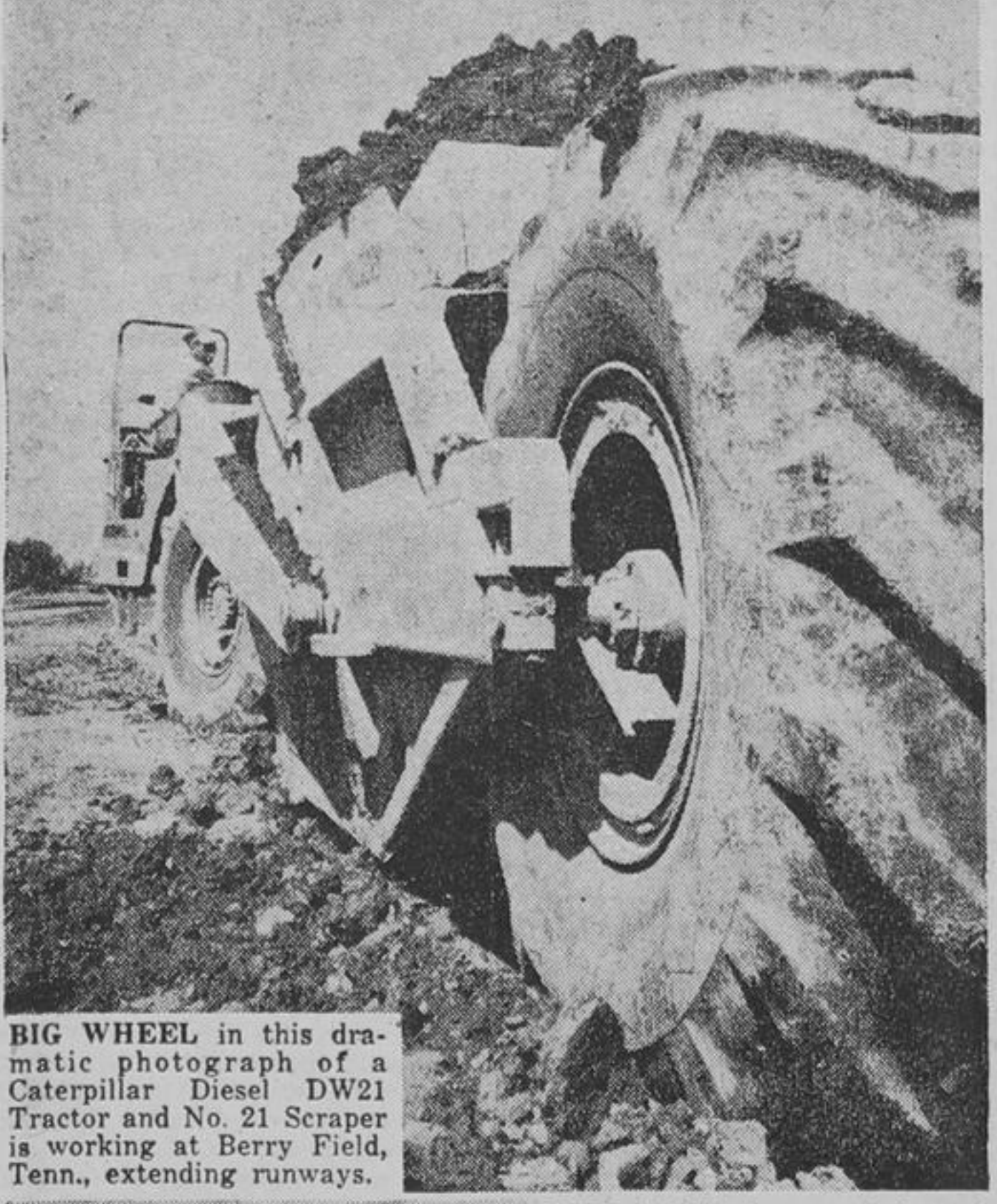
BIG WHEEL in this dramatic photograph of a Caterpillar Diesel DW21 Tractor and No. 21 Scraper is working at Berry Field, Tenn., extending runways.
