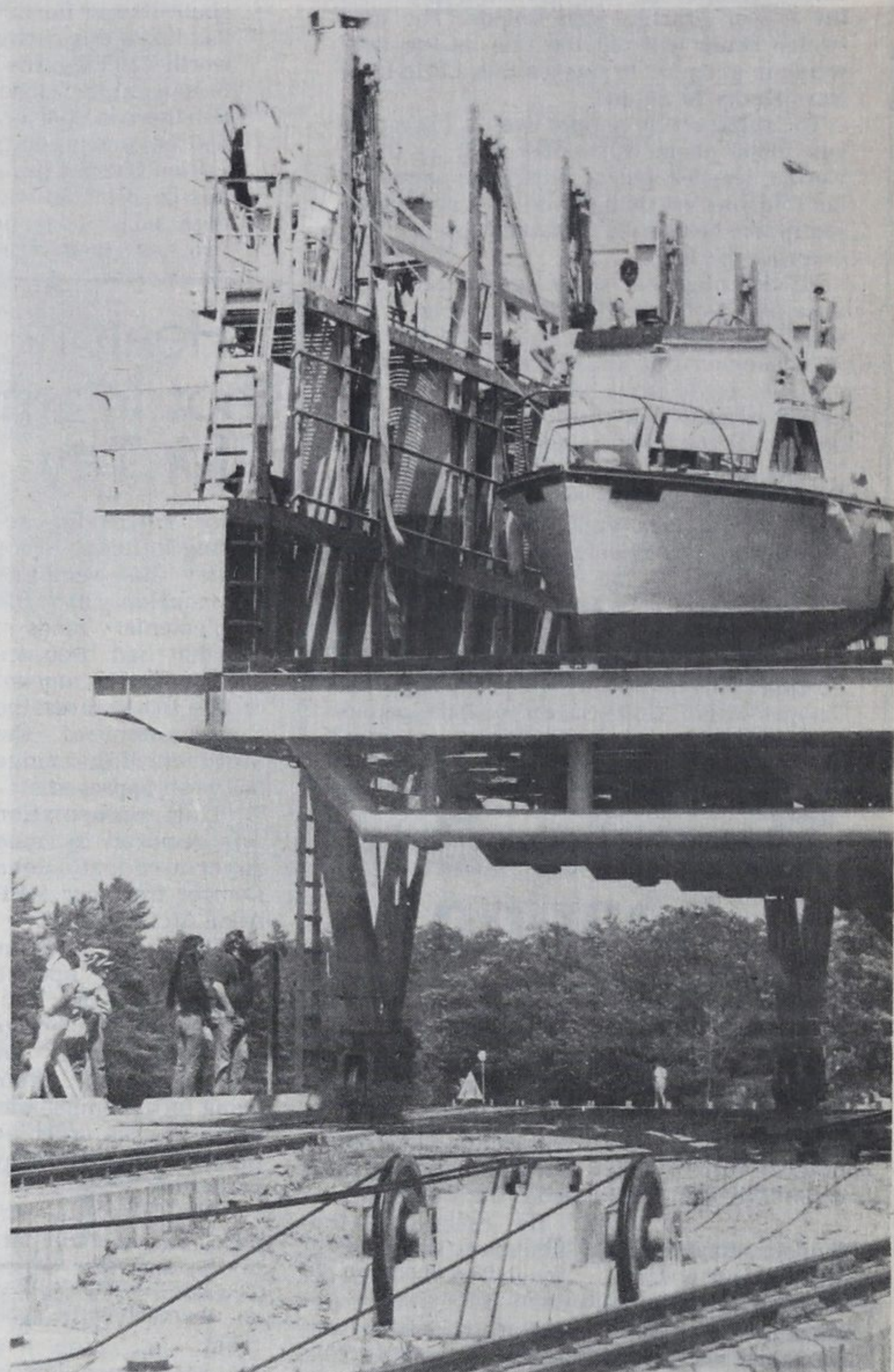
Marine railway in operation
