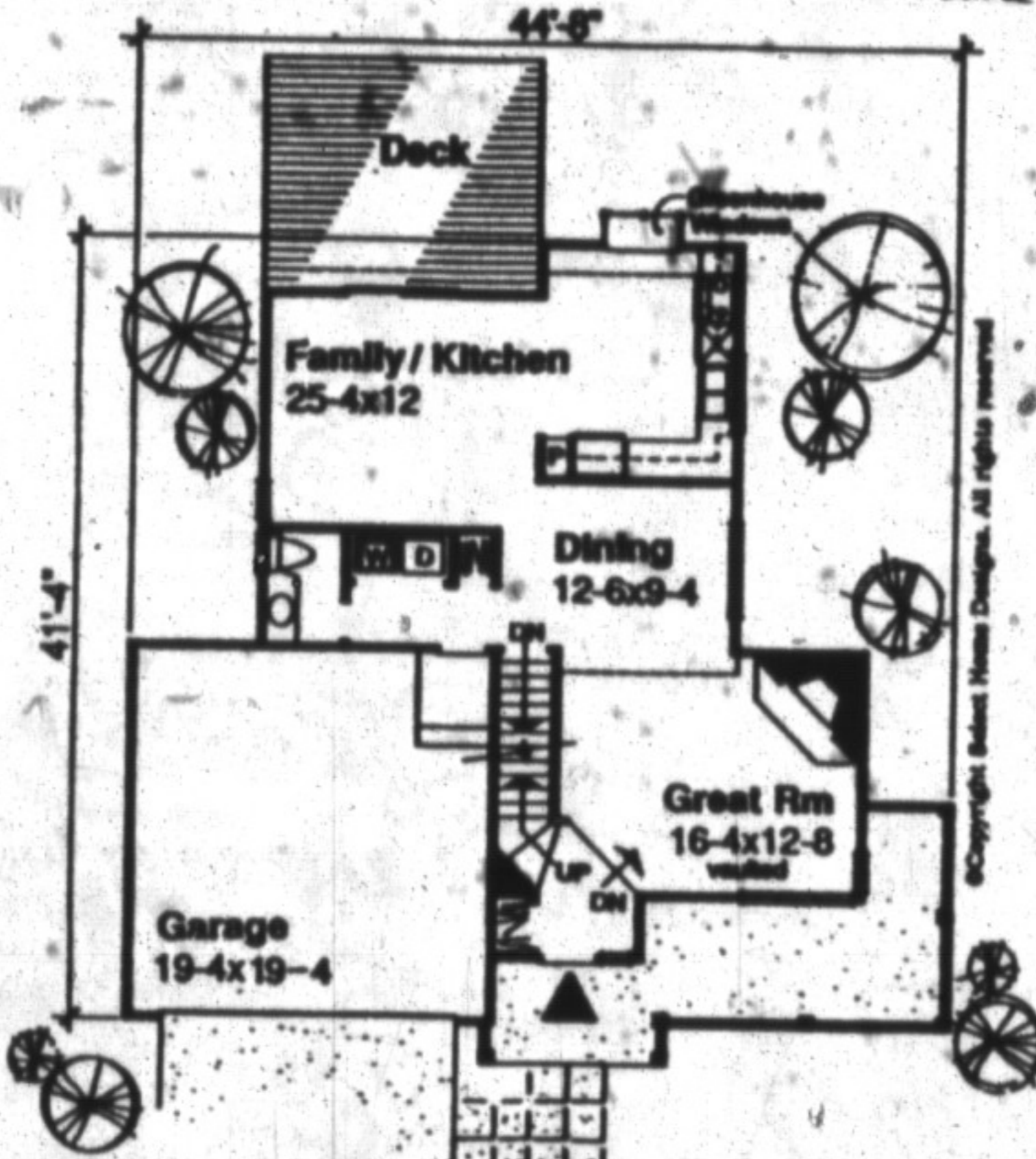
Plan No. 2095-1580
