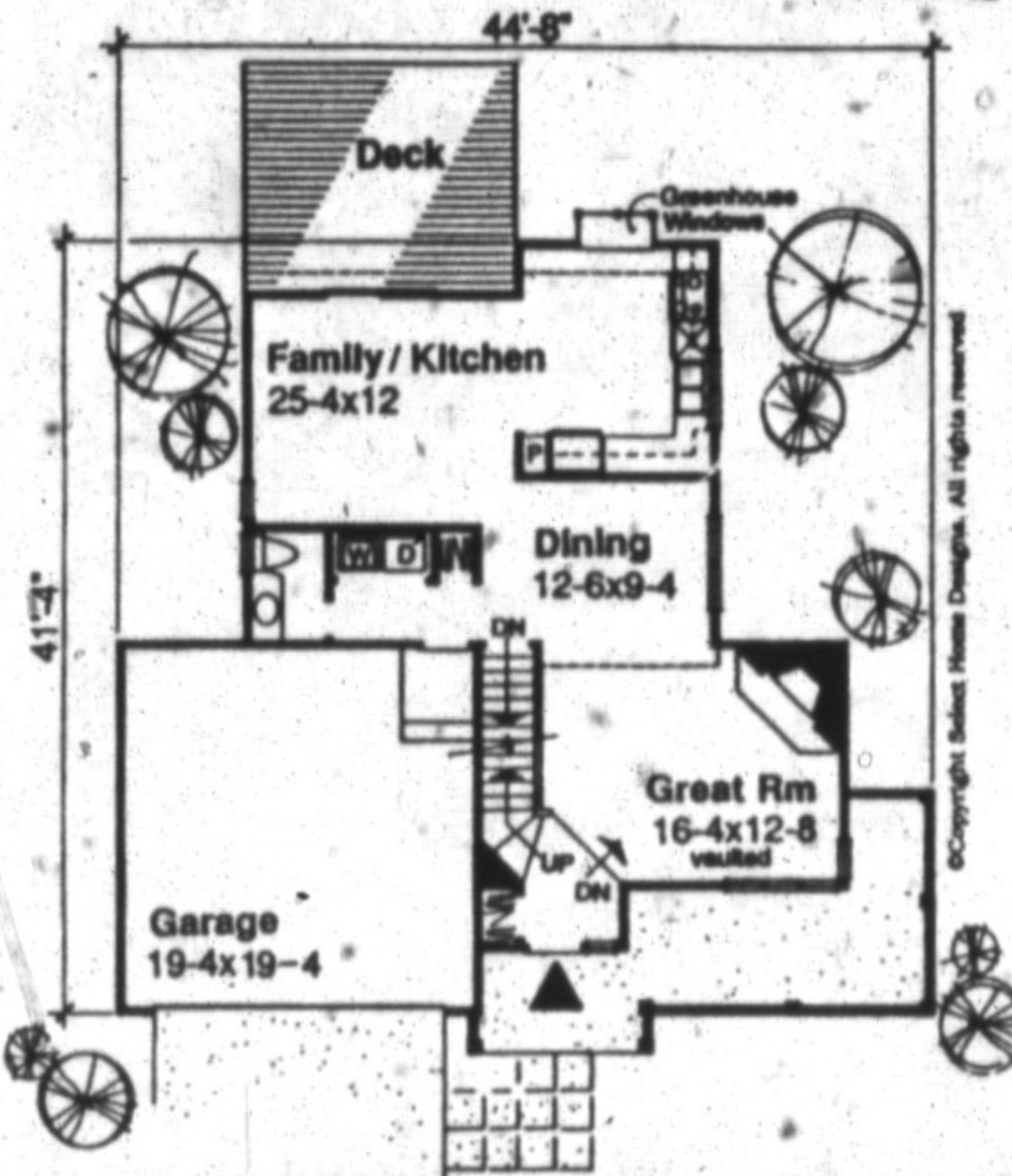
Copyright Select Home Designs. All rights reserved. Plan No. 2095-1550
