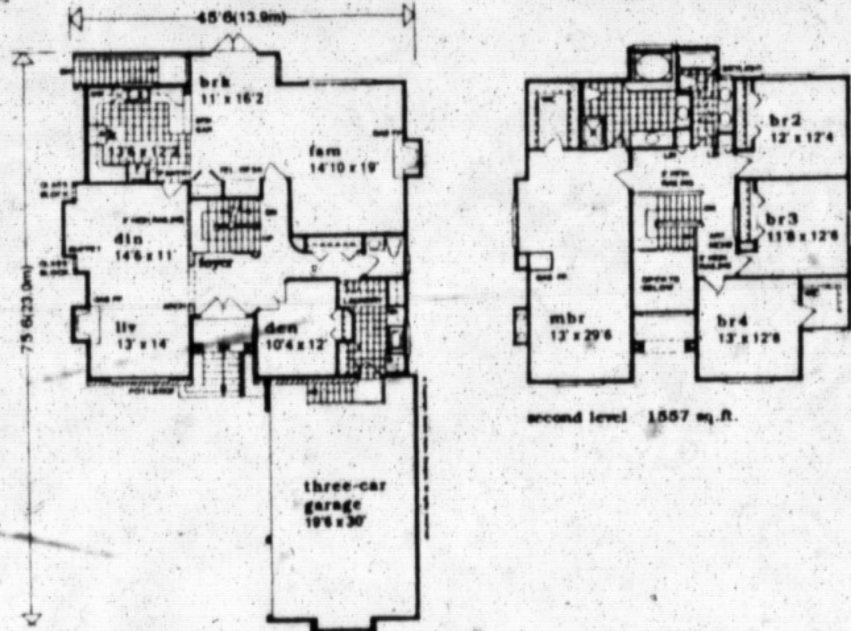
Plan No. 95-3207
