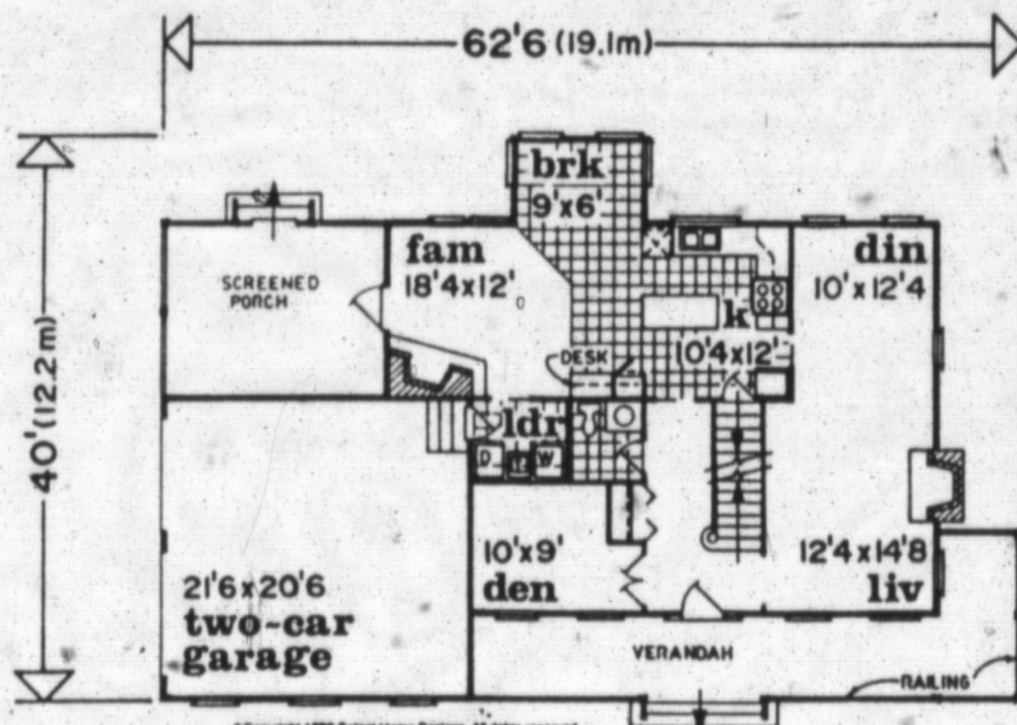
first level 1098 sq.ft.
