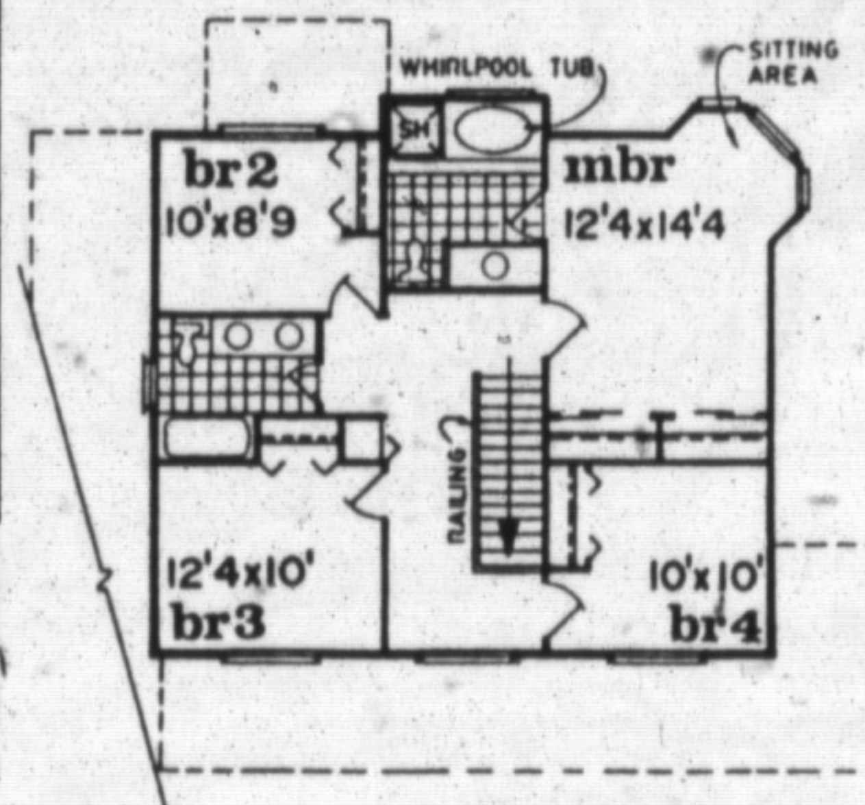
second level 996 sq.ft.
