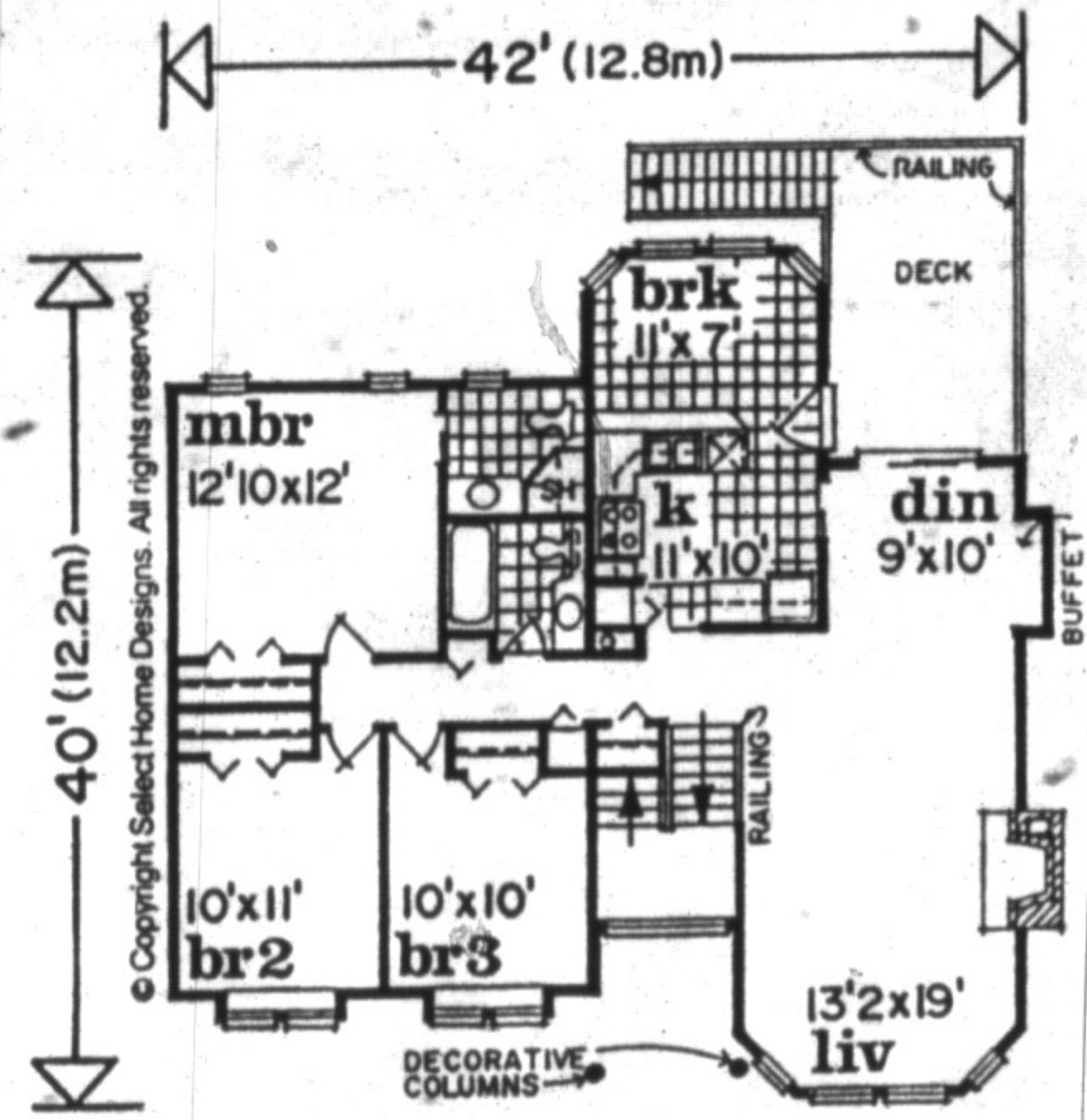
first level 1299 sq.ft.
