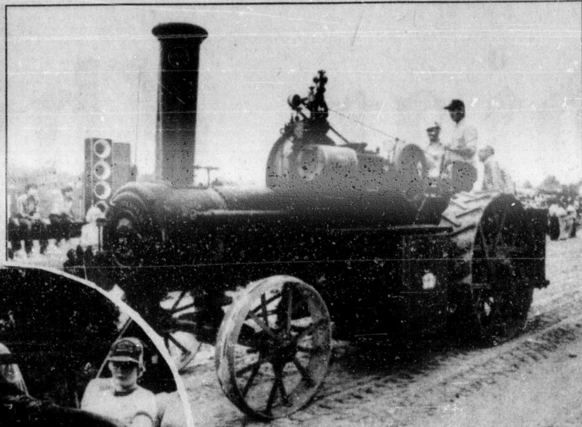
Unique machine. Bill Watson of Kilbride restored this George White steam engine by replacing the boiler with one from another steam engine.
