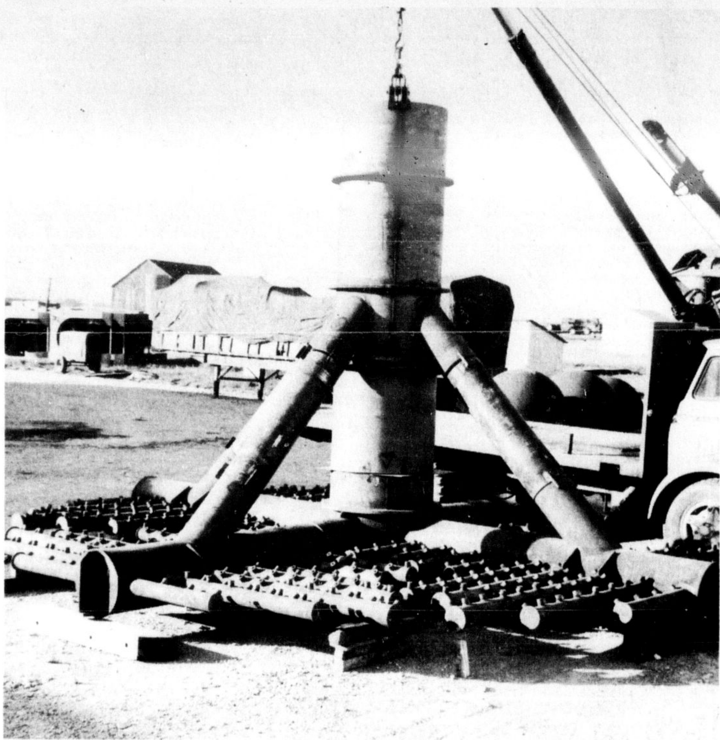
REGENERATOR AIR GRID was built by Kingsleigh Industrial, on Nipissing Rd. The grid, when ready will be installed in a petroleum refinery in Montreal. (Photo by J. Jennings)
