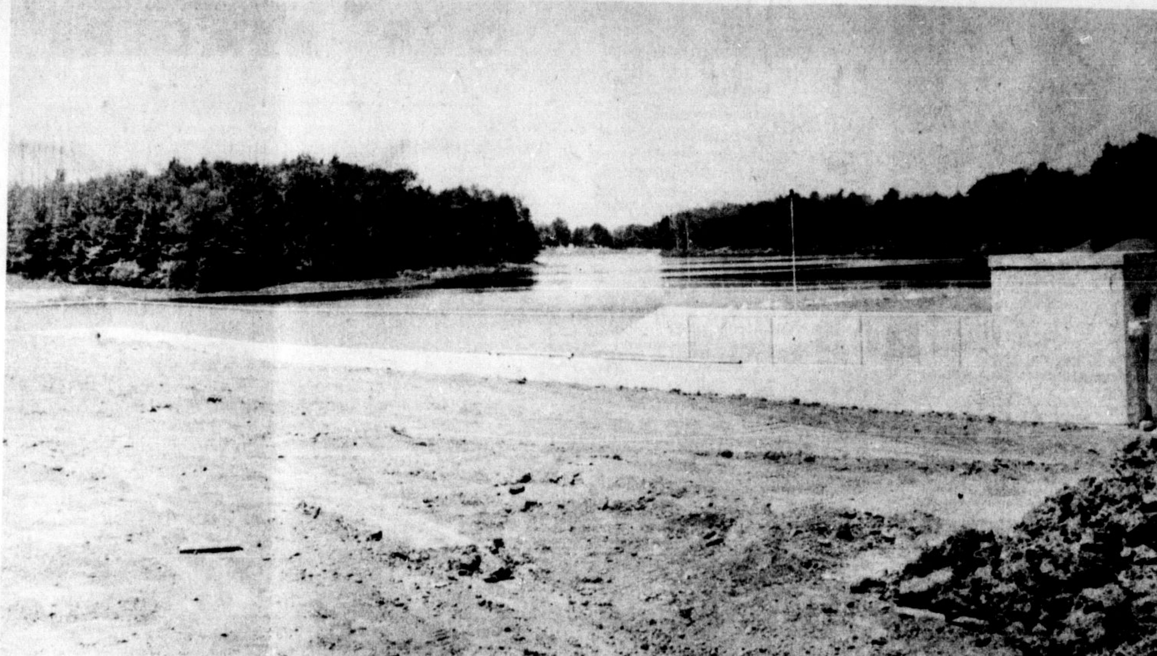
THE SCOTCH BLOCK DAM is filling up and creating a mile-long lake east of Highway 25 near Speyside. The project was built by Halton Region Conservation Authority as a summer stream control measure, and features a unique Fabri-Dam, an inflated rubber balloon to control the height of water in the dam. —(Staff Photo)
