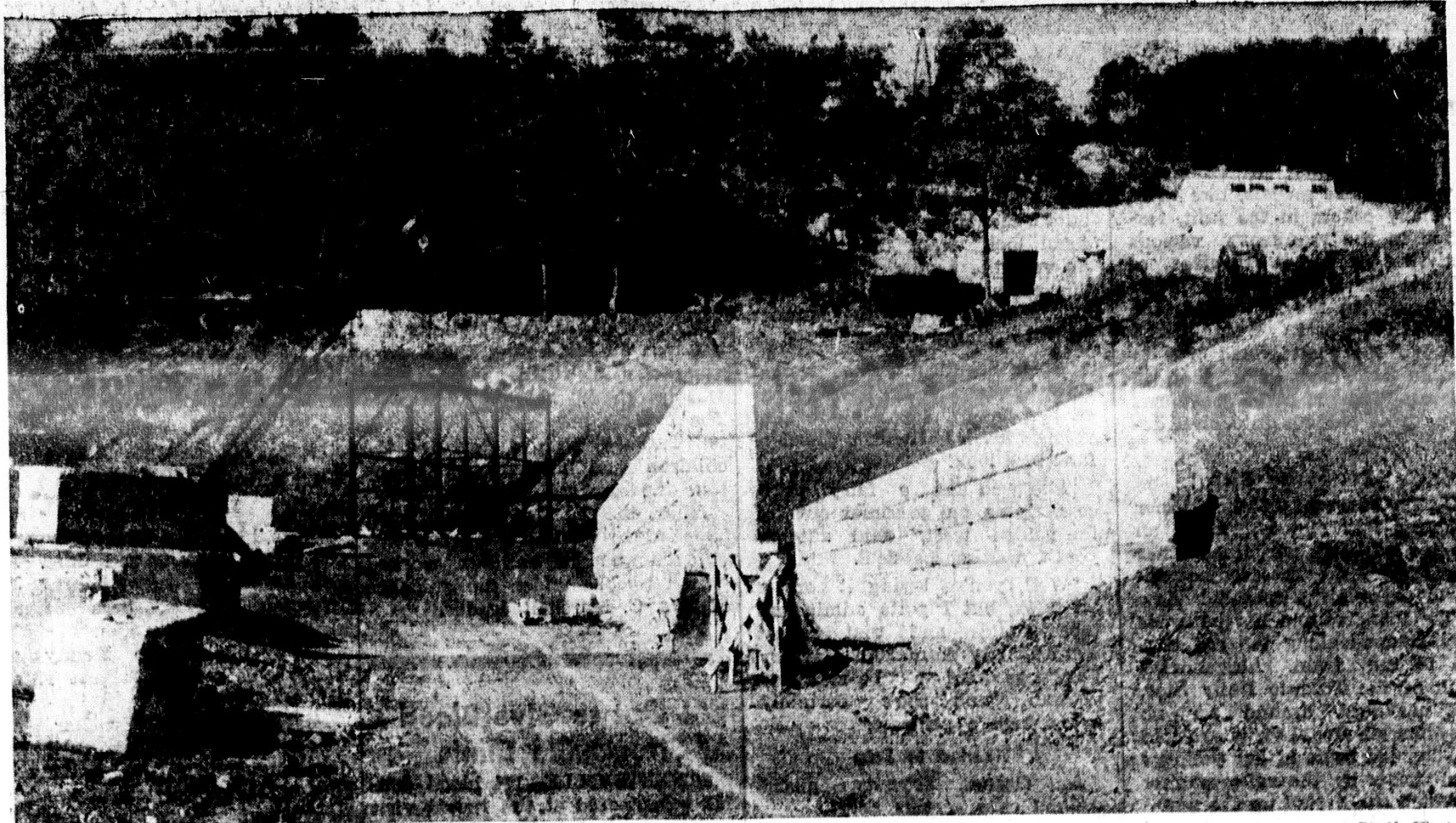
THE LOWER PLATEAU on the site being built by the Milton Quarries Ltd., will contain four secondary crushers, a stock pile and a huge steel screener. Shown above are bins that will feed the crushed stone to waiting trucks. The huge wall of stone will be a loading bin. It will contain approximately 150 pieces of stone that weigh six tons each. To the left of the stone structure workmen are busy building another steel bin.
