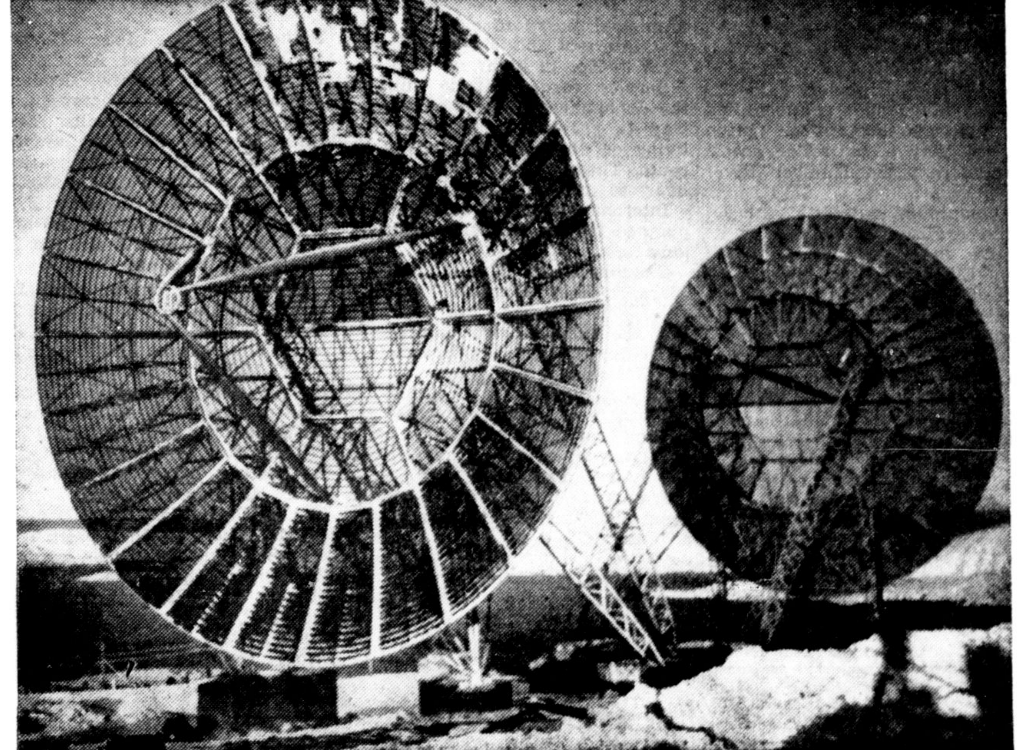
COMMUNICATIONS HISTORY has been made in Canada's sub-Arctic with the setting up of the world's first full-scale installation of over-the-horizon microwave transmission equipment, using the "tropospheric scatter" principle. The installation, employing huge dish-like antennae such as these, was built by The Bell Telephone Company of Canada's special contract department.
