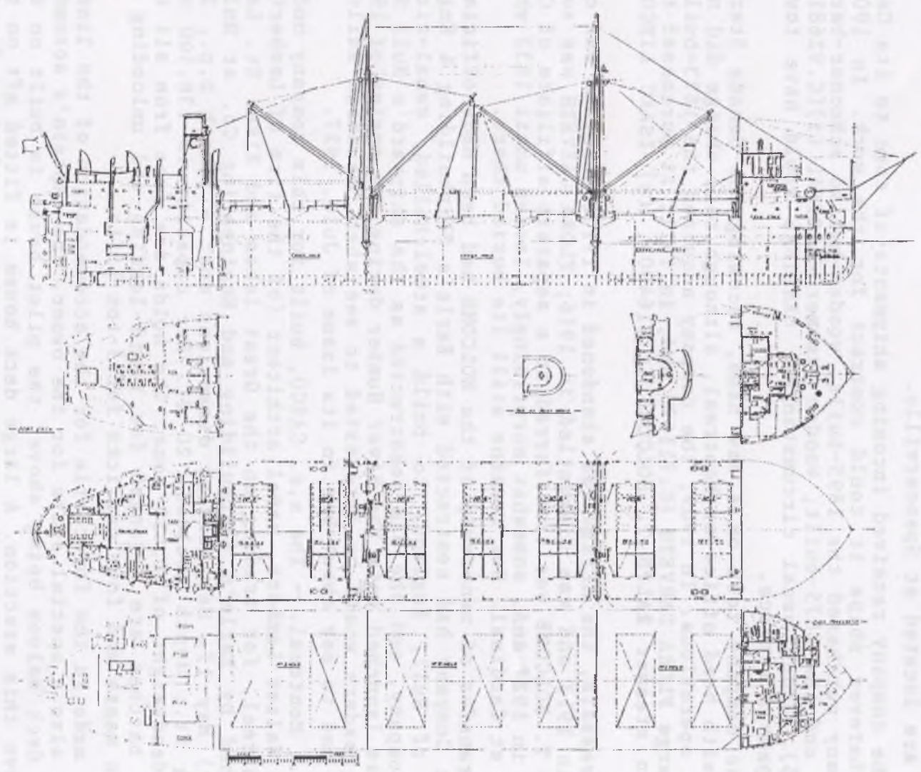
S.S. "CASCO" WELLAND CANAL TYPE VESSEL
