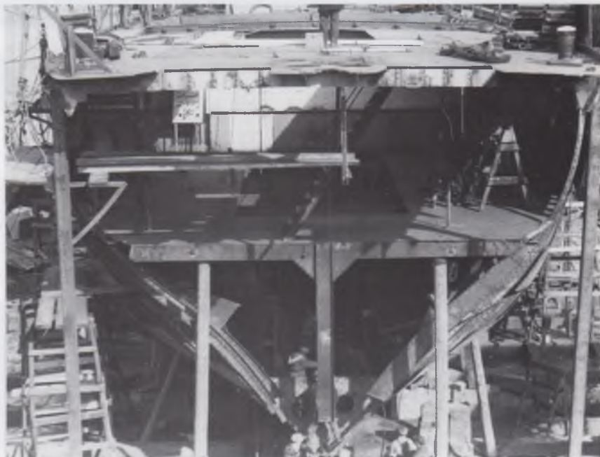
This view of BLACK RIVER on the drydock at Port Weller in 1952 shows her old stern cut away during the dieselization.
