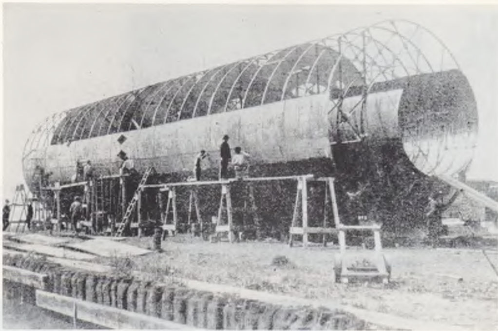
Knapp's ROLLER BOAT takes shape at the Polson shipyard during the summer of 1897.
