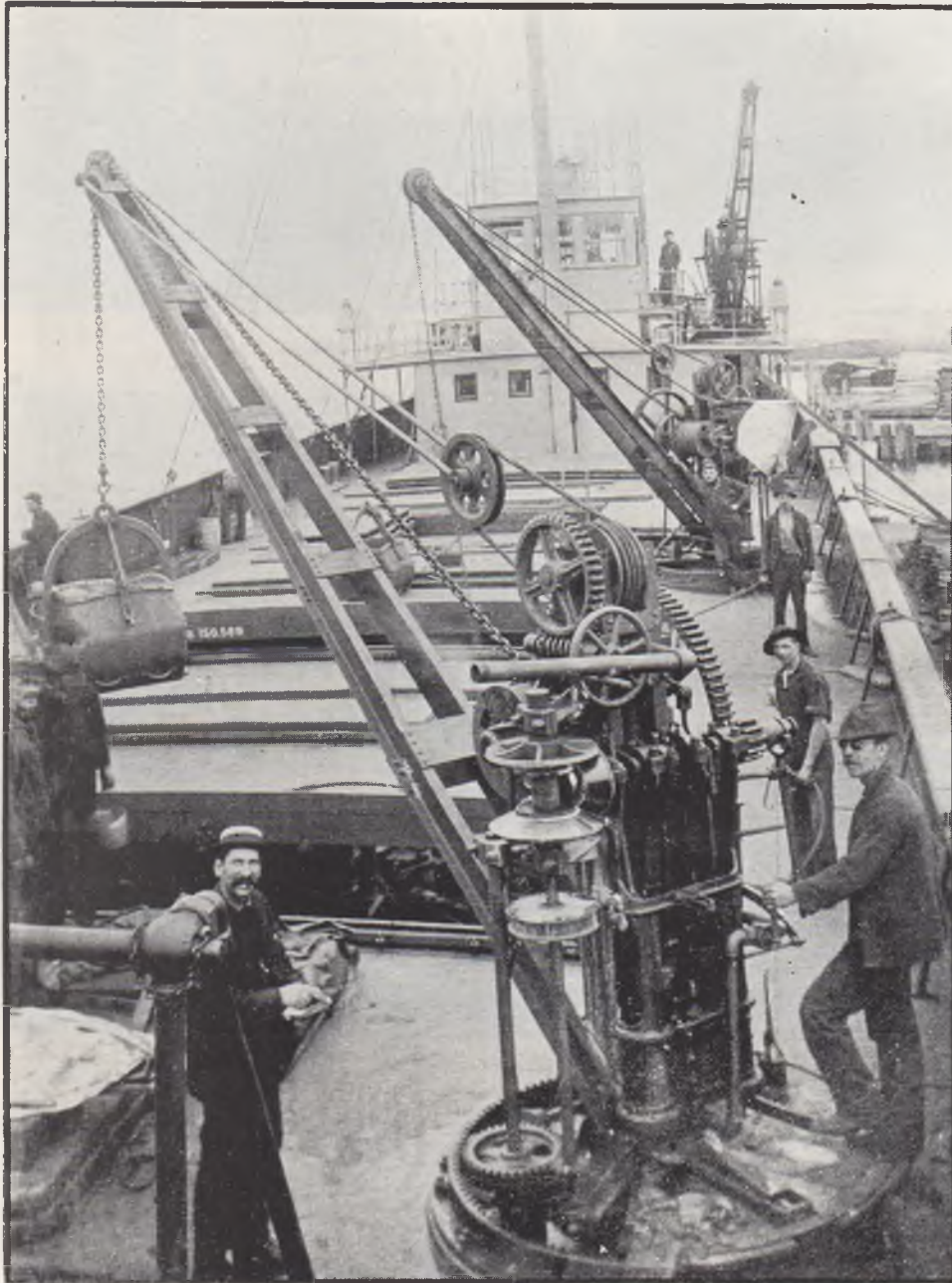
We promised our readers a view of the deck cranes on PIONEER/NATIRONCO, and here it is, as it appeared in "Around The Lakes", published in 1894 by the Detroit Drydock Company.
