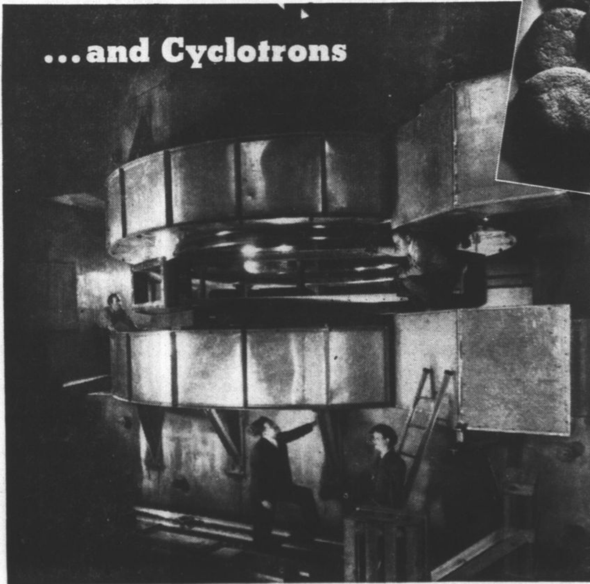
Synchro-cyclotron being installed by Institute for Nuclear Studies, University of Chicago, at a cost of $2,200,000.
