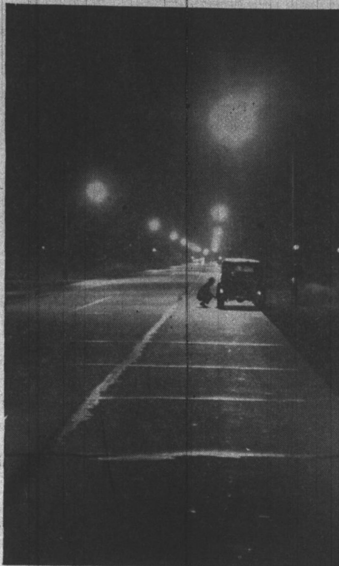
Camera portrays safety feature of new sodium vapor highway lighting installed by the Public Service Company of Northern Illinois on a demonstration mile of U. S. 41 near Northbrook. (Left) man and car are practically invisible although within range of ordinary auto lamps. (Right) same situation revealed by sodium vapor highway lighting. Both views are from identical spots, with same camera exposures. Safety experts agree that proper highway lighting is an important factor in cutting the heavy accident toll attributed to night driving hazards.
