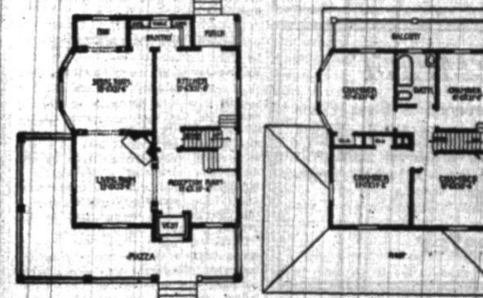
FIRST FLOOR PLAN. SECOND FLOOR PLAN.
