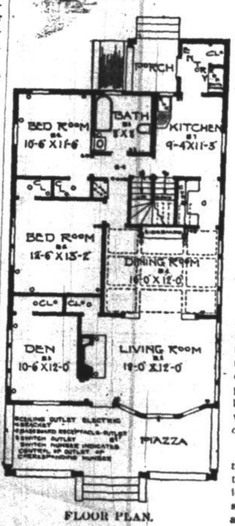
FLOOR PLAN.
